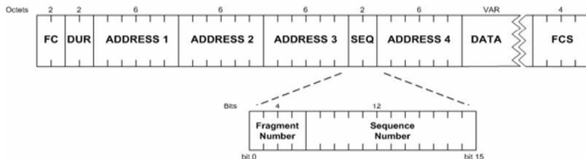
Fig. 3.2 Basic WLAN Frame sequence number
