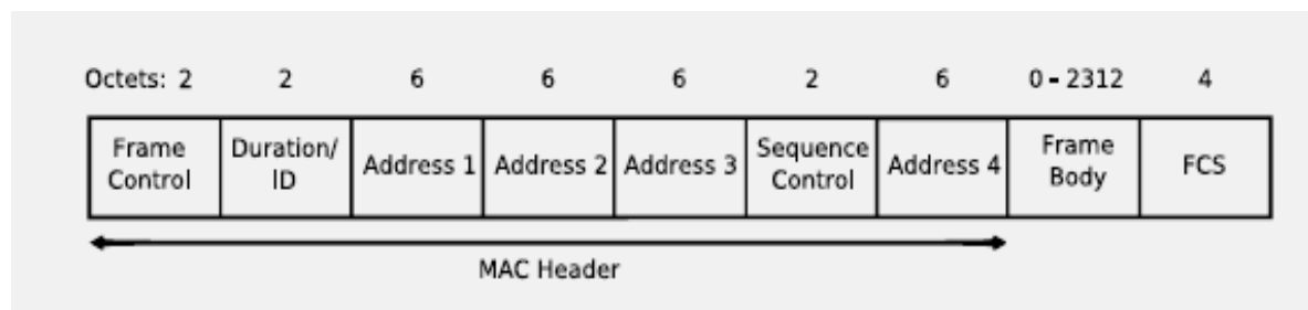
Fig. 3.1 Basic WLAN MAC Frame Format [3]
