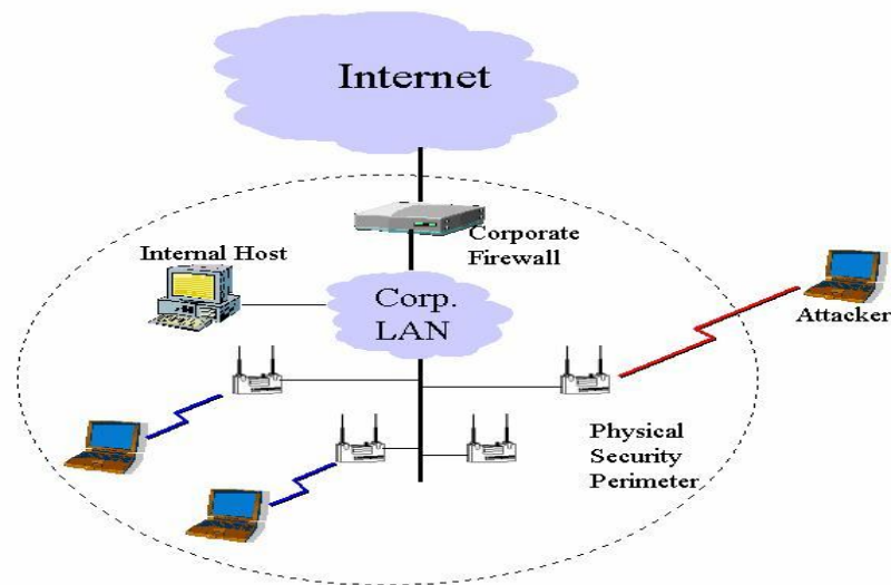
Fig. 4.1 Parking Lot attacker in WLAN
