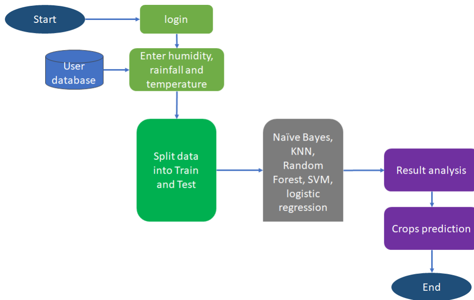
Figure 3.7: Proposed Prediction Model
