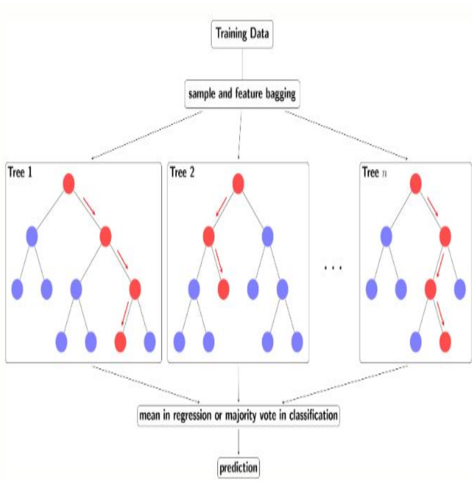
Figure 2.8: Random Forest
