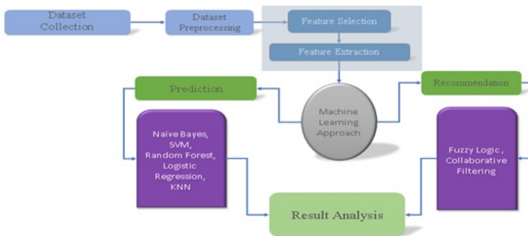
Figure 3.1: Proposed Model
