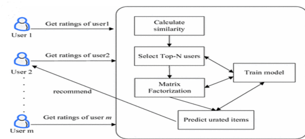
Figure 2.10: Collaborative Filtering
