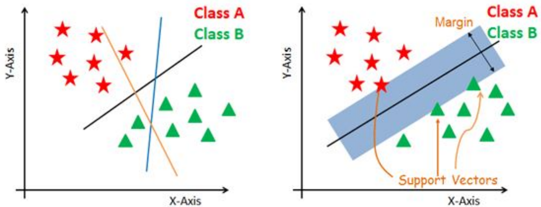
Figure 2.7: Creation of Hyperplane
