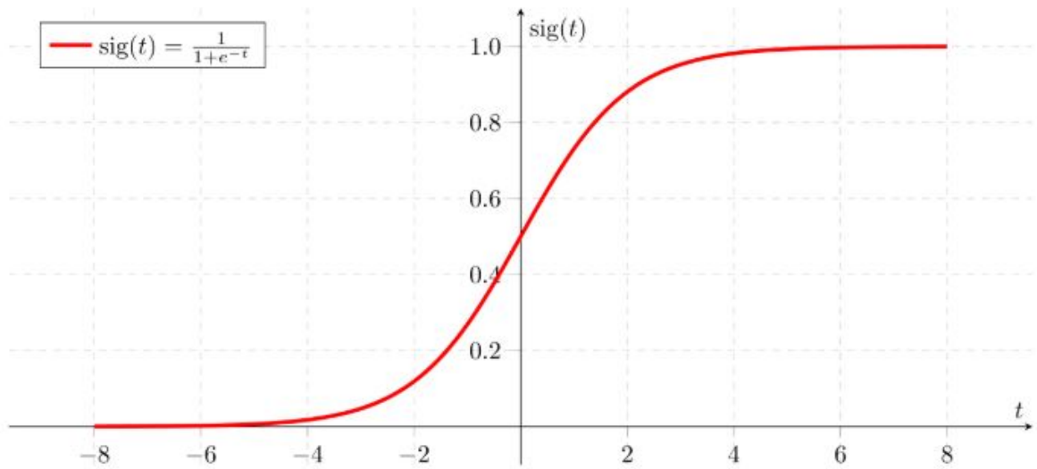
Figure 2.2: Sigmoid Curve
