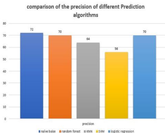
Figure 4.1: Precision comparison of different Prediction Algorithms
