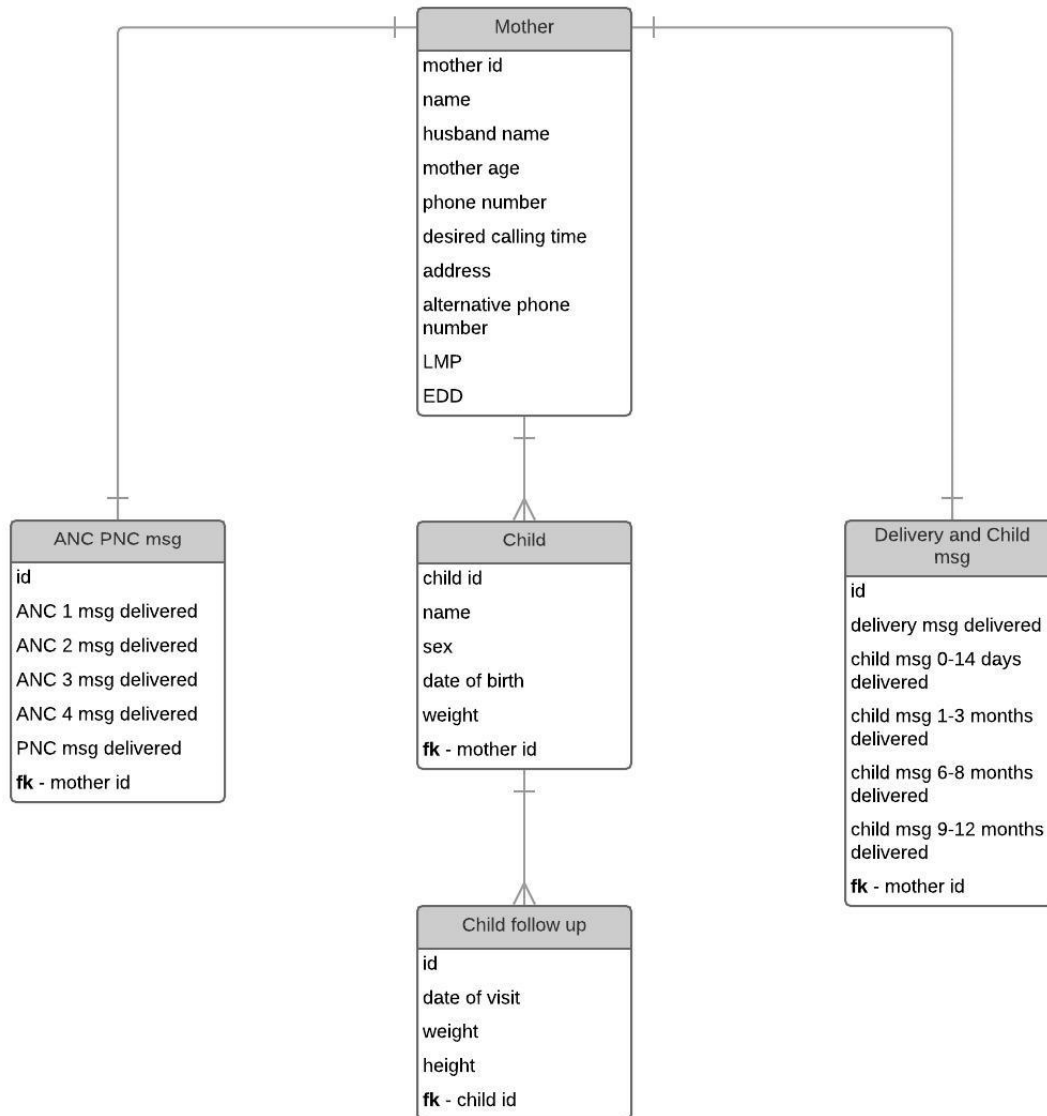
Fig 3.3.1: Entity relationship model
