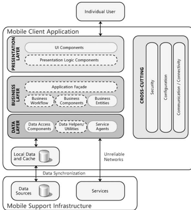
Fig 3.2.1: The typical structure of a mobile application
