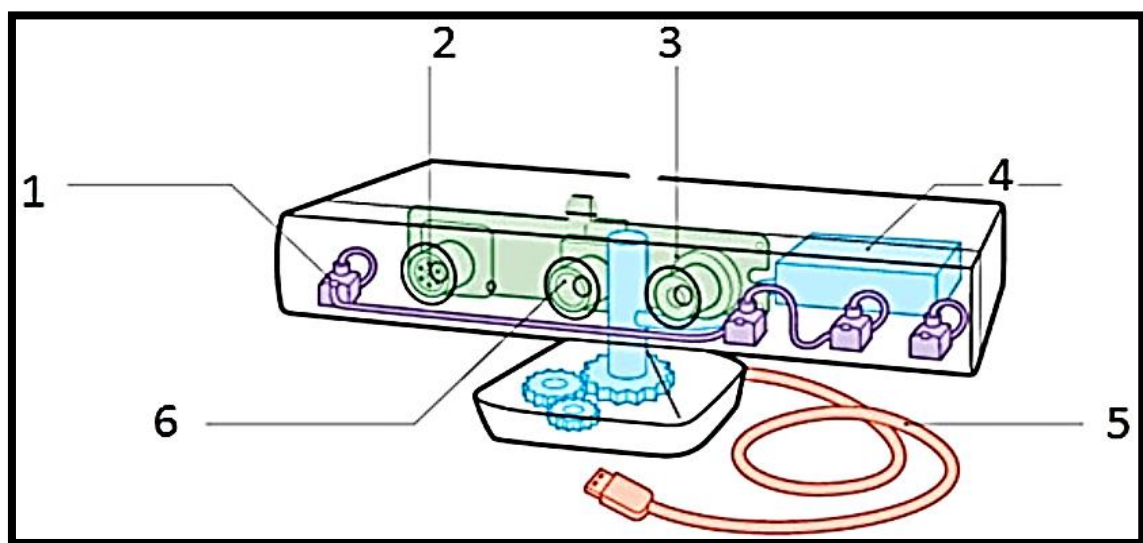
FIGURE 1:KINECT WITH KEY COMPONENTS(1.MICROPHONE ARRAY, 2. IR EMITTER, 3. DEPTH CAMERA, 4. TILT MOTOR, 5. USB CABLE, 6. COLOR CAMERA)
