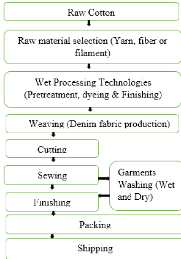
Figure 2.1. Process Diagram of Composite Textile Factory
