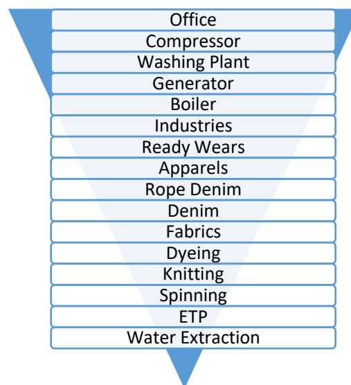
Figure 3.3. Conceptual Model for Energy Efficiency in RMG Factory
