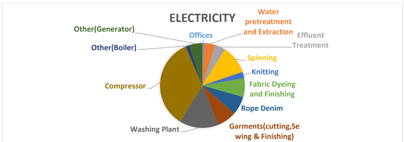
Figure 2.3. Pie chart of electricity consumption in percentage of utilities of the factory.
