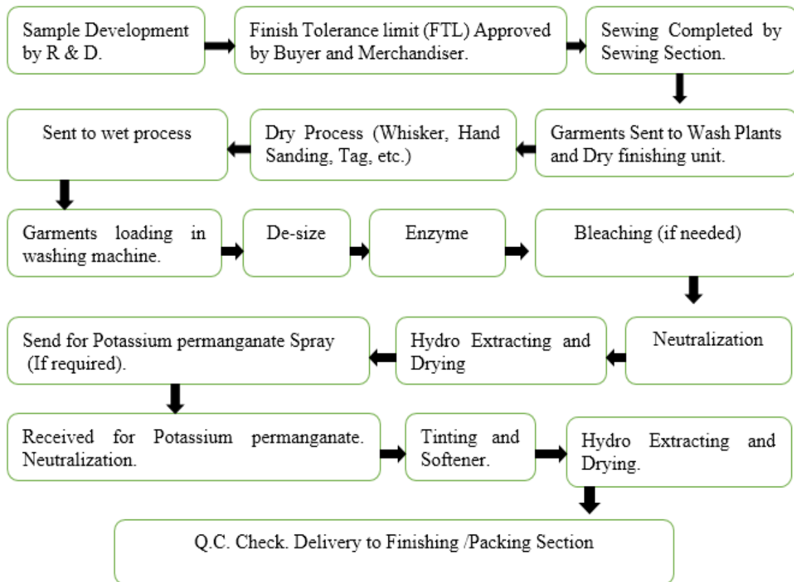
Figure 2.2. Process flow diagram of washing.
