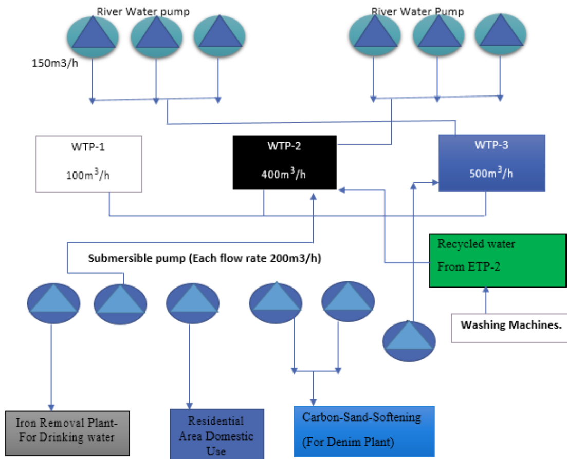
Figure 4.5. Water Distribution diagram.
