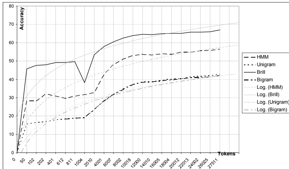
Figure 9: Performance of POS Taggers for Telugu [Test data and Tagset source: [41]]
