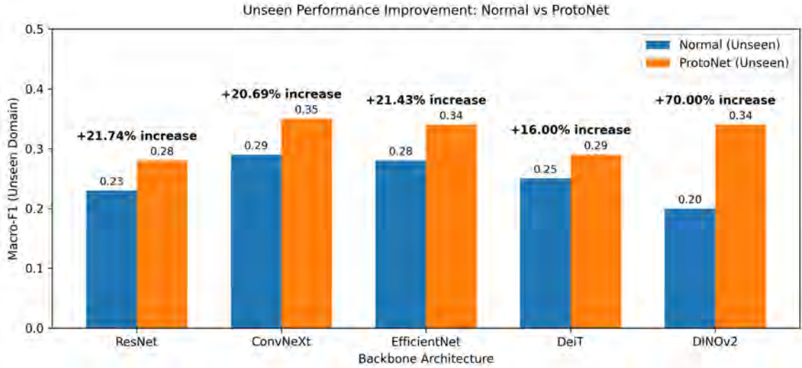
Figure 5.3: Cross domain performance improvement with meta learning
