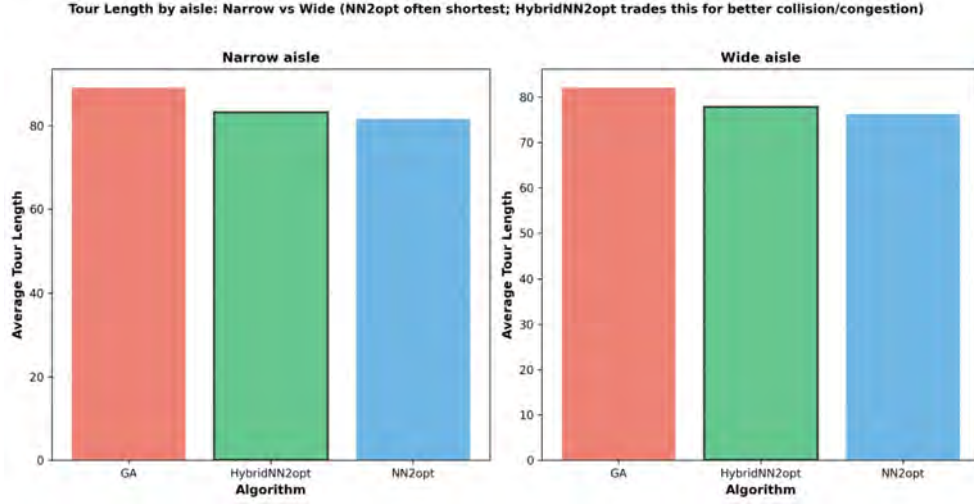
Figure 5.5: Comparison of Average Tour Length
