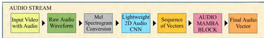
Figure 4.4: Simplified pipeline of the Audio Stream.
