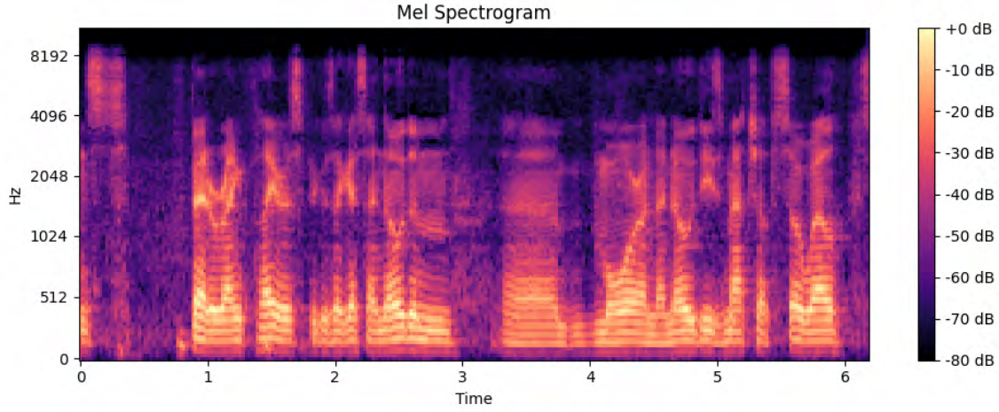
Figure 4.5: Mel spectrogram representation of a sample audio clip from the AV Lips dataset. The horizontal axis represents time (in seconds), the vertical axis represents Mel-frequency bands (ranging from 0 to 8 kHz), and the color intensity indicates the magnitude of frequency components (in dB), with warmer colors representing higher energy. The spectrogram captures the temporal-spectral characteristics of speech, revealing formant structures and temporal variations that are essential for audio-visual synchronization detection.
