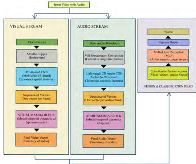
Figure 4.2: Proposed architecture of our Dual-Stream Mamba Fusion Network
