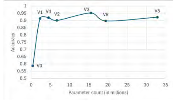
(b) Trend-line of accuracy scores with increasing parameter count.
