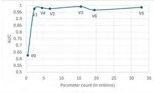
(a) Trend-line of AUC scores with increasing parameter count.
