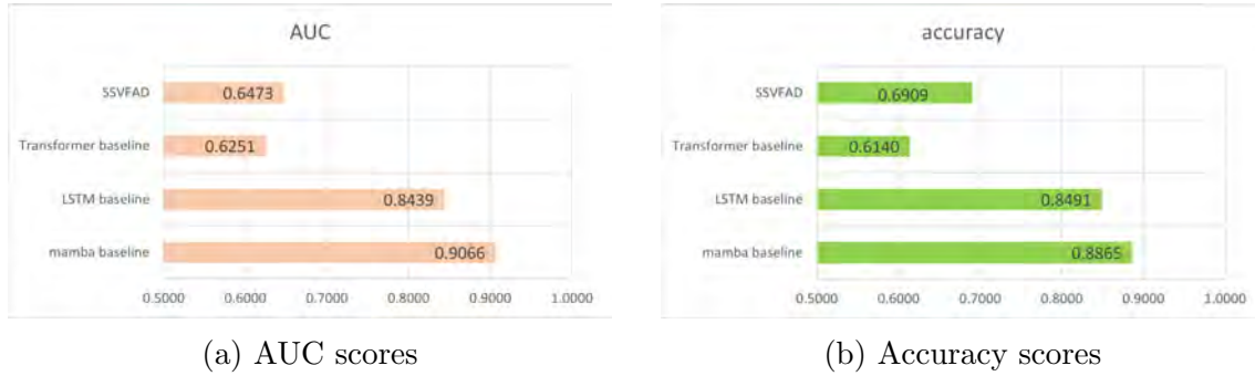
Figure 5.3: The performance metric of the four models when trained on the AV Lips dataset, but evaluated on the FakeAV Celeb dataset.
