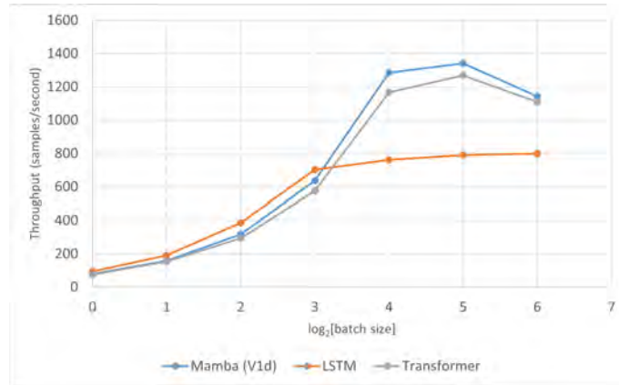
Figure 5.6: A graphical plot of the throughput values (in samples per second) of all the models except SSVFAD. SSVFAD had been negated in this graph for its much more explosive increase in throughput with respect to batch sizes, as evident in Table 5.7
