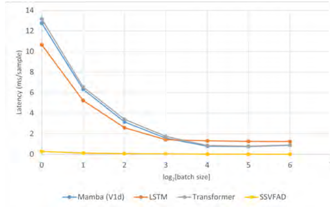
Figure 5.5: A graphical plot of the latency values (in milliseconds per sample) vs \log_2[\text{batch size}] across different batches of all the models.
