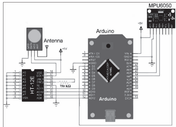
Fig. 2. The gesture recognizer hand module with transmitter and encoder.
