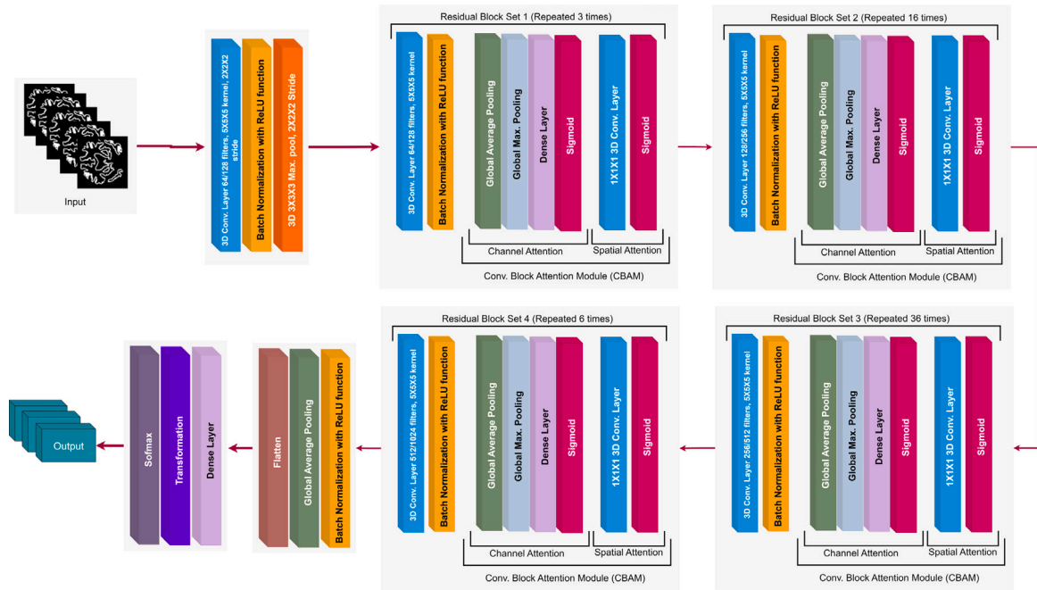
Fig. 5. Visual illustration of 3D-ResNet architecture.
