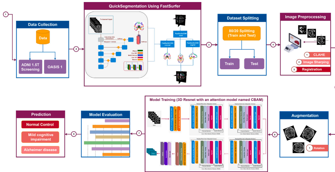
Fig. 1. Overall pipeline for detection of Alzheimer's disease from 3D MRI.
