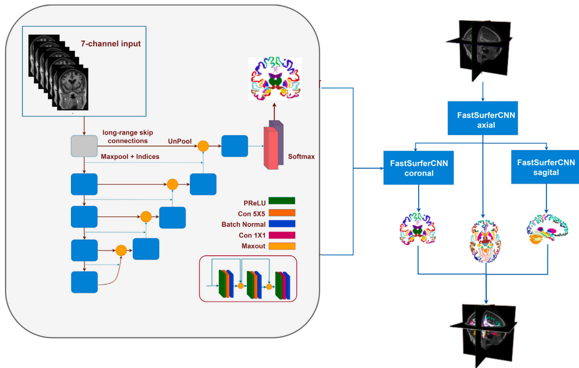
Fig. 2. Visual illustration of FastSurfer QuickSeg.
