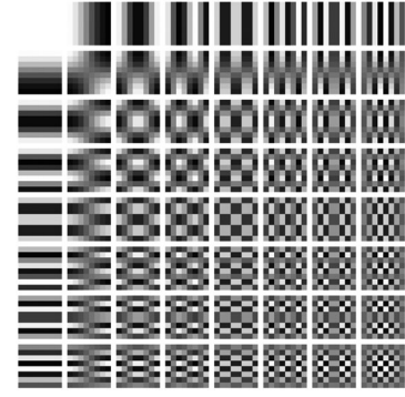
Fig. 3. Discrete cosine transform (DCT) [25].
