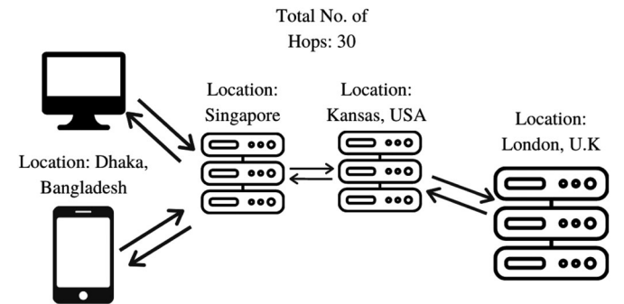
Fig. 8. Testbed server setup to obtain performance of diversified remote devices using the web hosting server.
