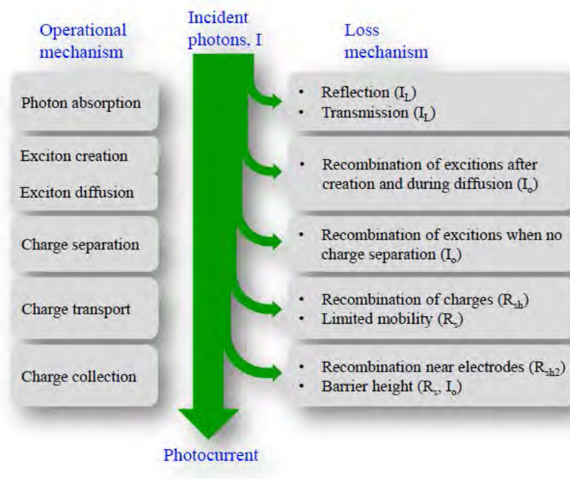
Figure 4: Operational steps and loss mechanism in organic solar cell
