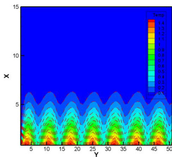
FIGURE 26 Isothermal lines for several values of G_r (fluid view)
