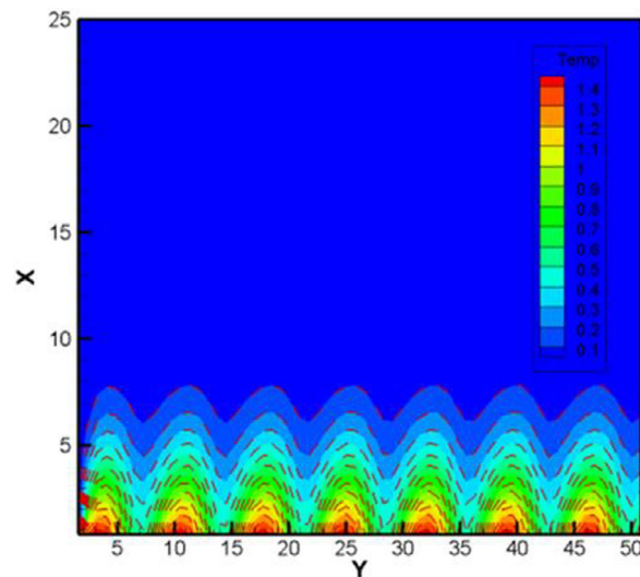
FIGURE 28 Isothermal lines for different values of R_d (flood view)
