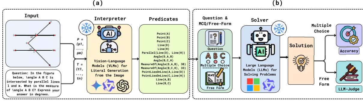
Figure 1: (a) An Interpreter Agent generates formal predicates from images and questions using VLMs. (b) A Solver Agent then solves the problem using these predicates as LLM input.
