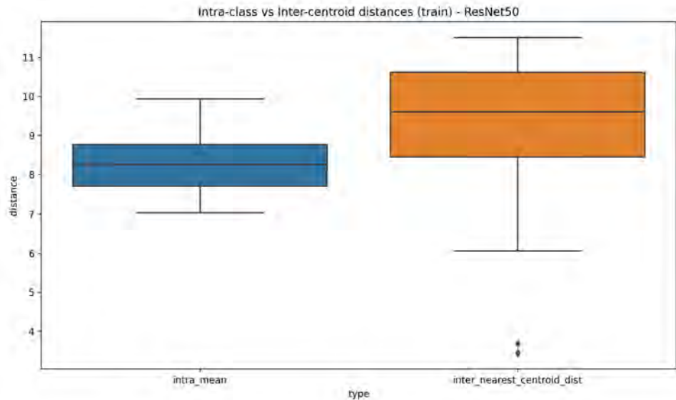
Figure 5.6: Intra-class vs. nearest Inter-class distances for ResNet50 embeddings.
