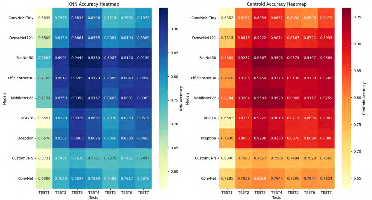
Figure 5.9: Heatmap of Black Background Dataset.
