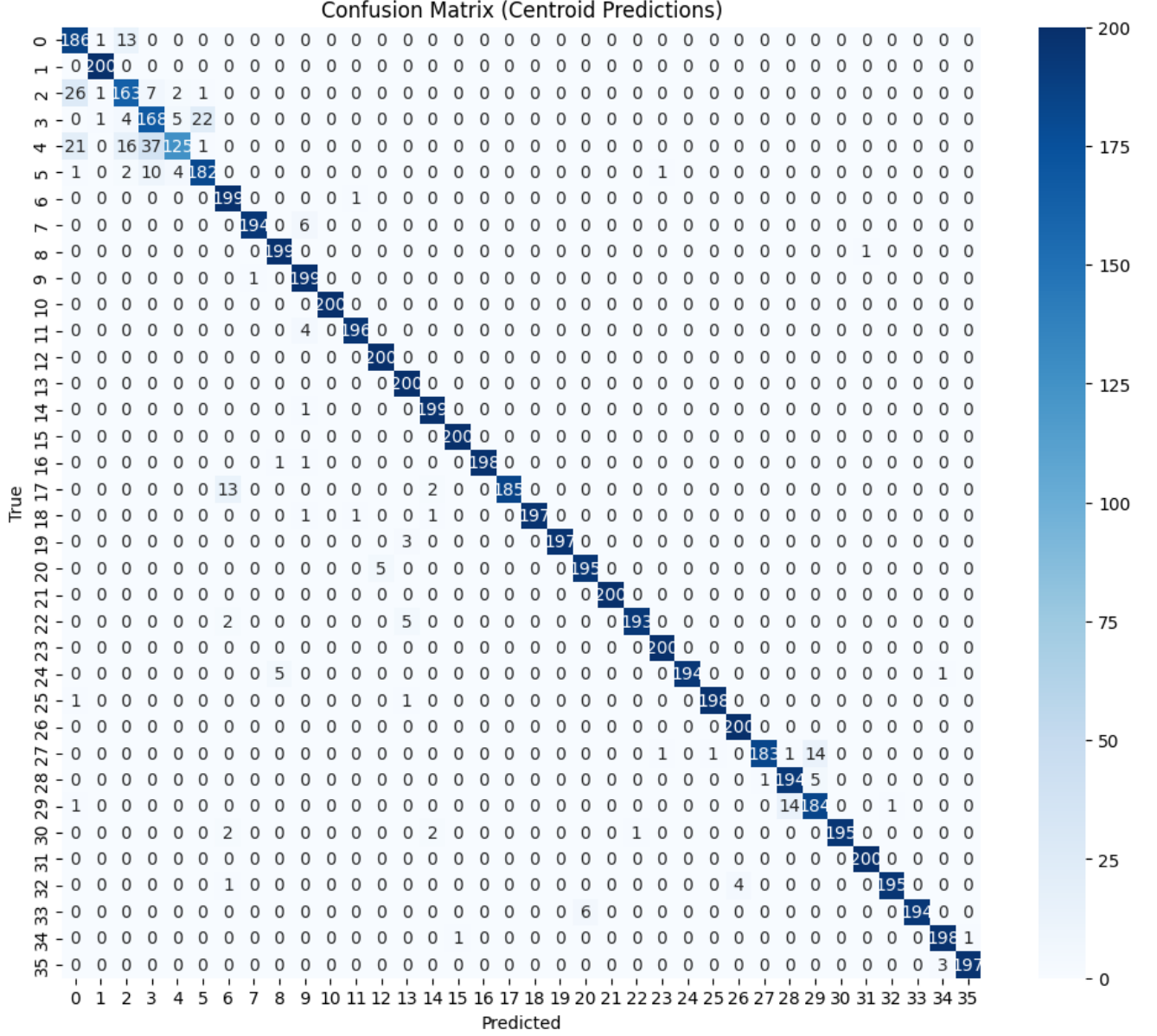
Figure 5.1: Confusion Matrix of ResNet50.
