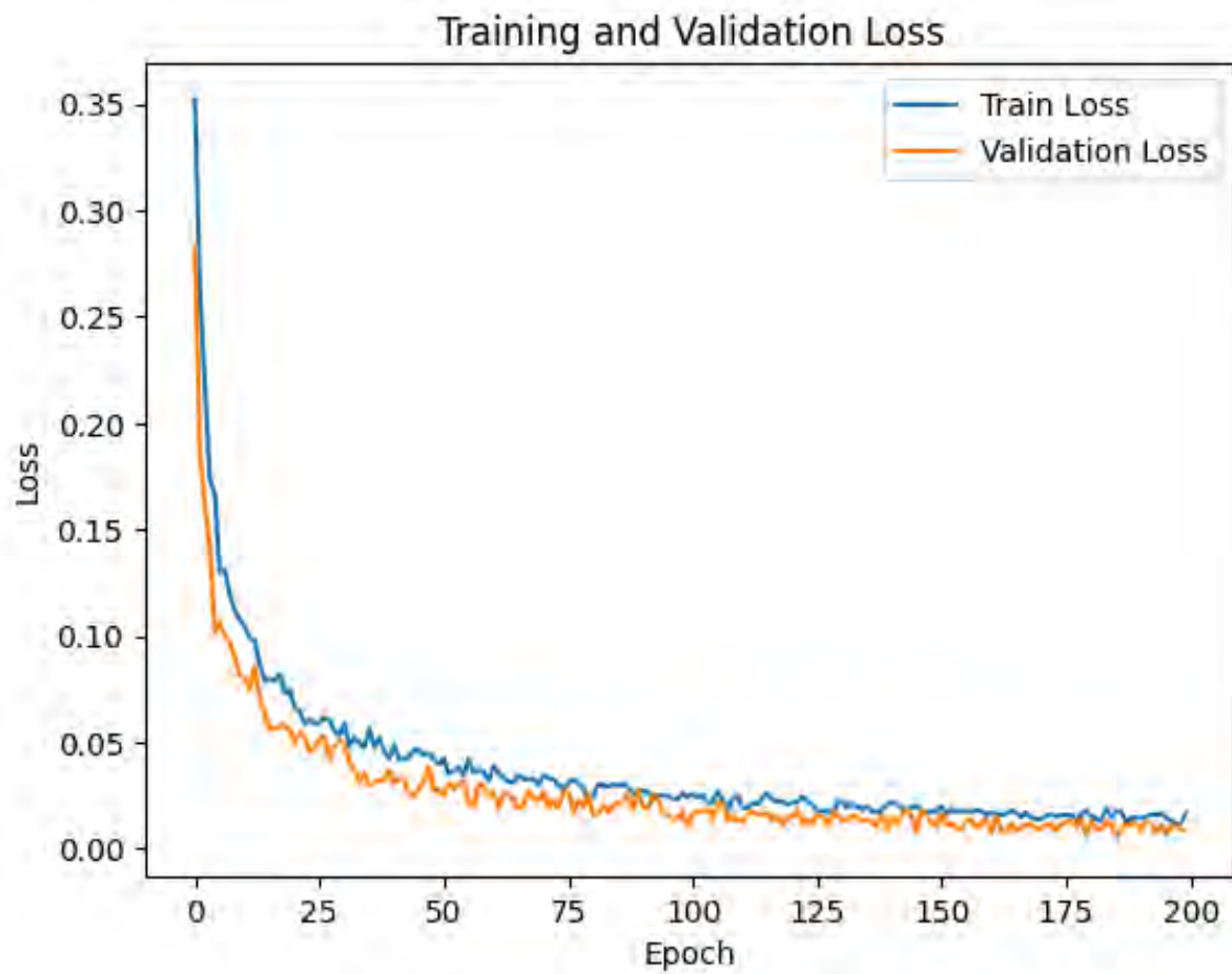
Figure 4.7: Training and Validation Loss of ResNet50
