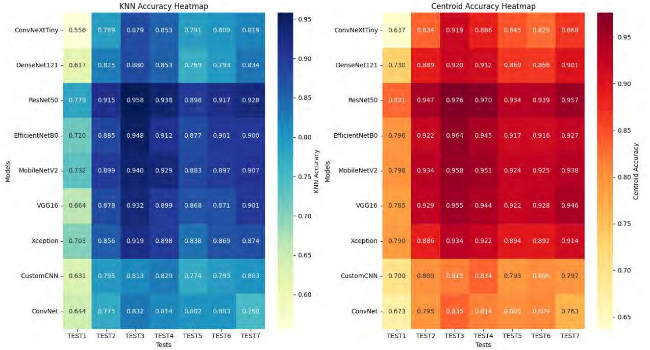
Figure 5.8: Heatmap of Background Dataset
