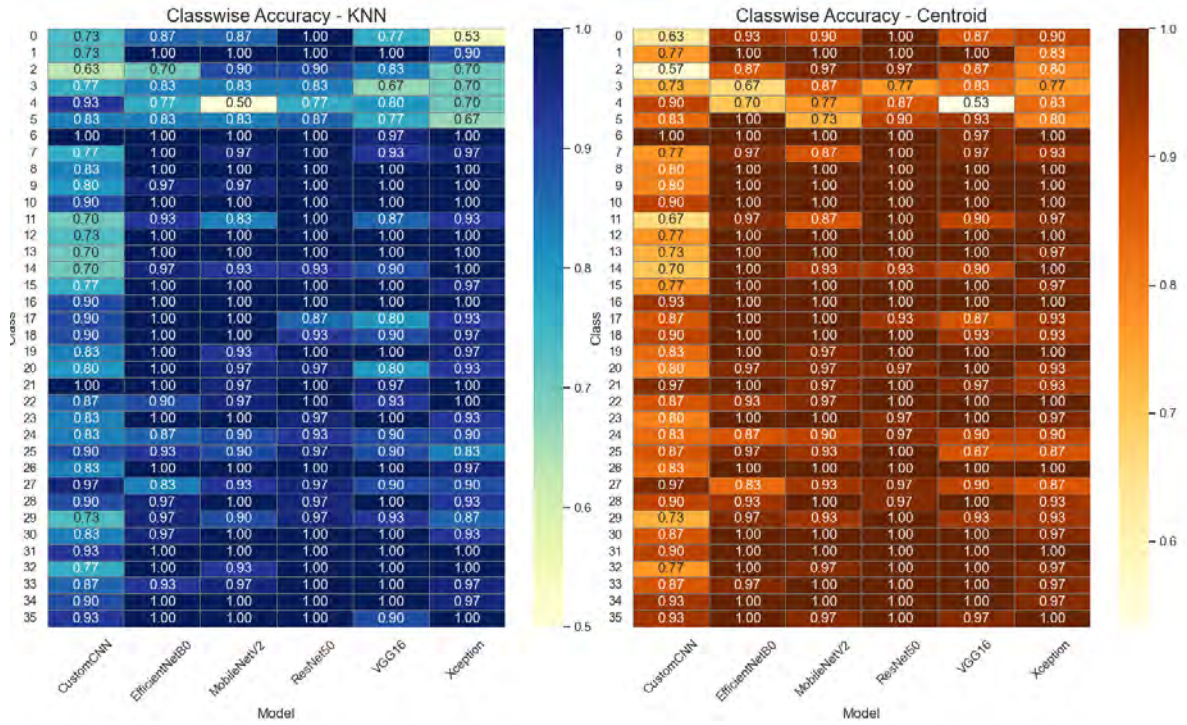
Figure 5.3: Classwise accuracy of best 6 model
