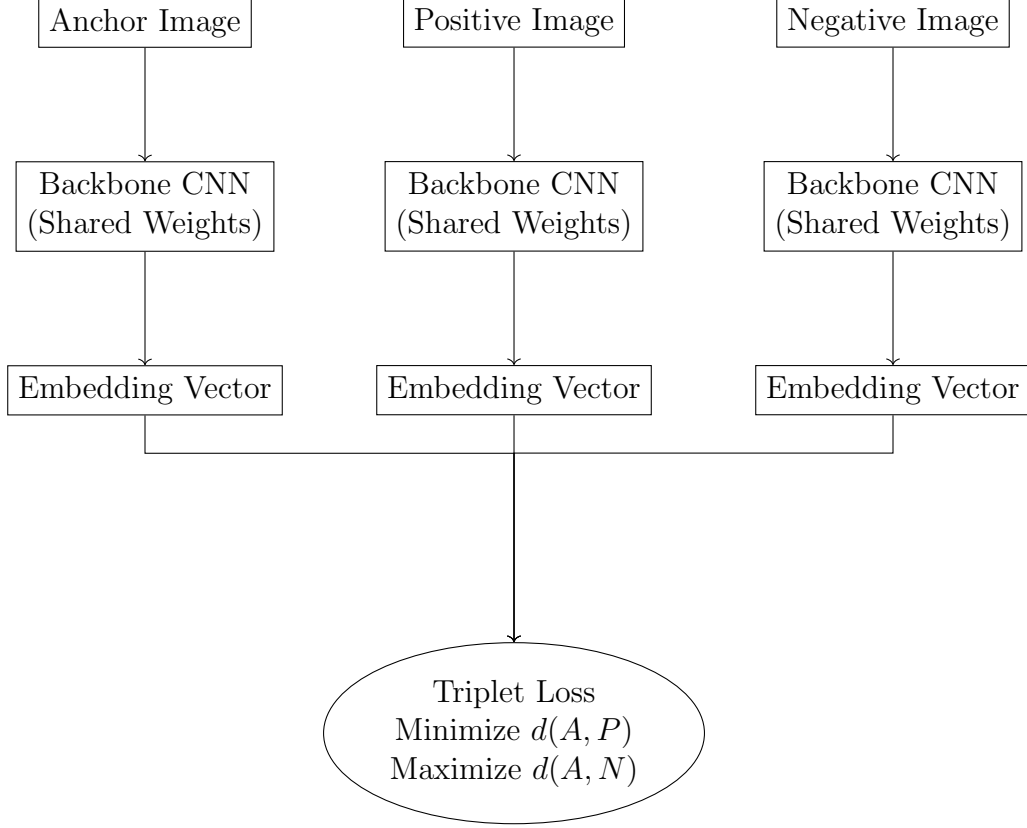
Figure 4.1: Triplet Network Architecture: Anchor, Positive, Negative inputs and Embedding Output
