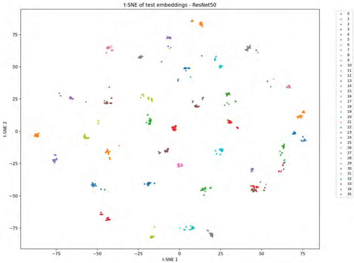
Figure 5.7: t-SNE visualization of test embeddings colored by class.
