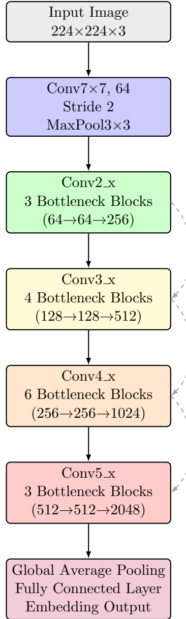
Figure 4.8: ResNet-50 architecture used for Bengali Sign Language gesture correction.
