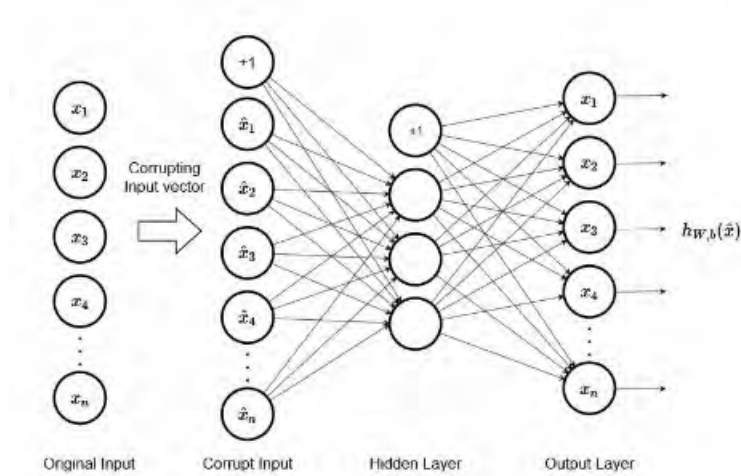
Figure 3.3: SDAE Architecture
