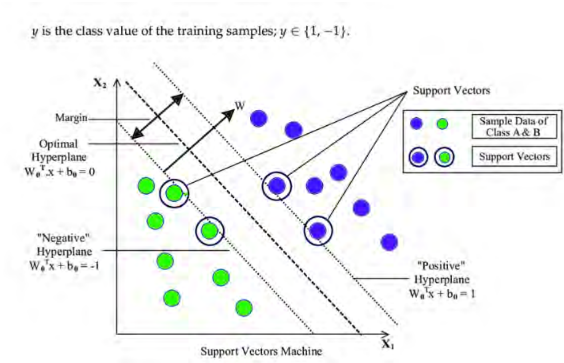
Figure 3.7: SVM Mechanism
