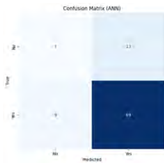
Figure 6.16: KPCA+SDAE -ANN
