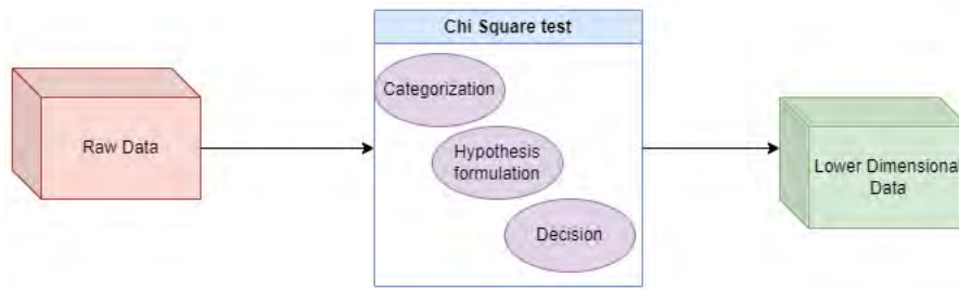
Figure 5.2: Feature Selection(Chi-square)
