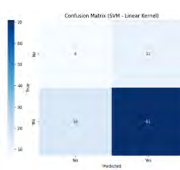
Figure 6.11: FS+SDAE SVM
