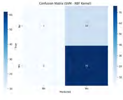
Figure 6.12: FS+SDAE SVM-RBF
