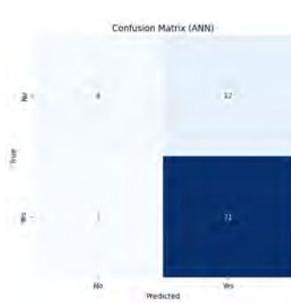
Figure 6.10: FS+SDAE-ANN
