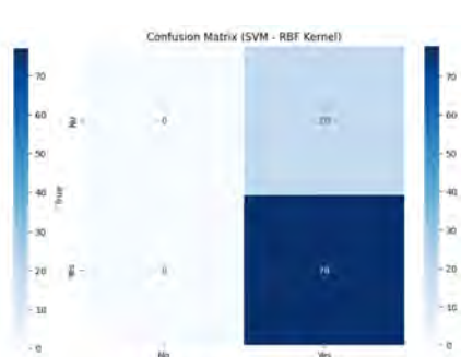
Figure 6.18: KPCA +SDAE SVM-RBF
