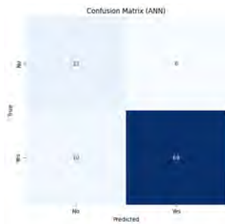
Figure 6.13: PCA+SDAE -ANN
