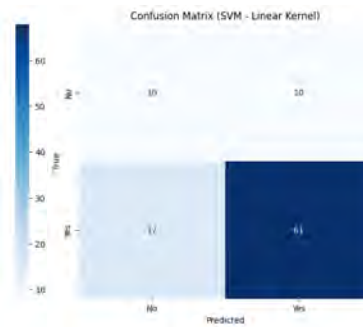
Figure 6.14: PCA+SDAE SVM
