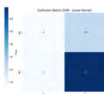
Figure 6.17: KPCA+SDAE SVM
