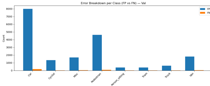
Figure 6.5: False Positive vs False Negative Bar Chart (Hybrid Model)
