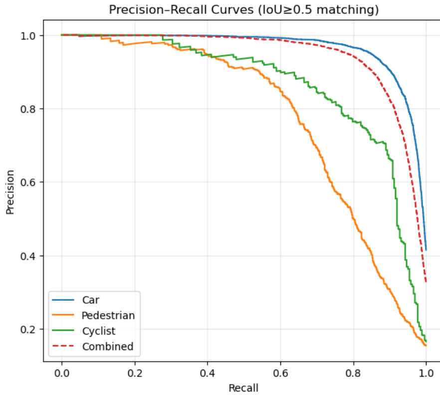
Figure 6.3: Precision-Recall Curves (Hybrid Model)
