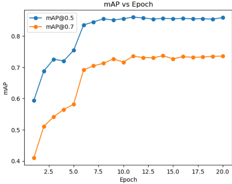
Figure 6.13: mAP vs Epoch (Faster R-CNN)
