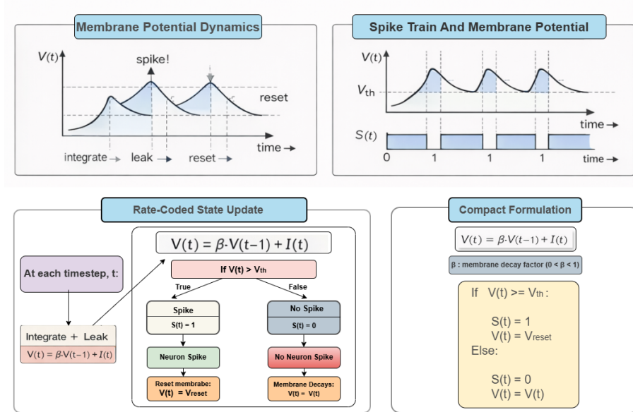
Figure 5.2: Internal Dynamics of LIF neuron illustrating membrane integration, spike generation and reset mechanism over time
