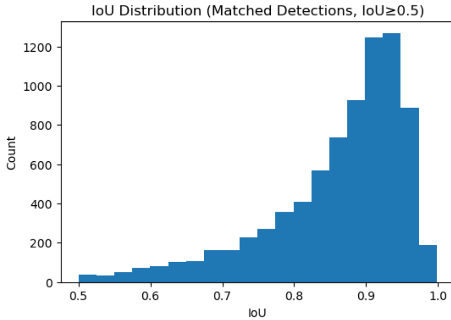
Figure 6.21: Histogram of IoU distribution (Faster R-CNN)
