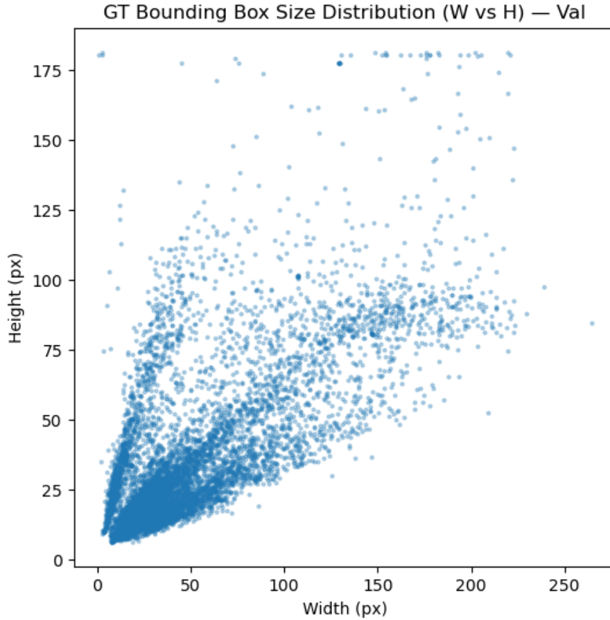
Figure 6.18: Ground truth bounding box size distribution for the KITTI validation set (Faster R-CNN)
