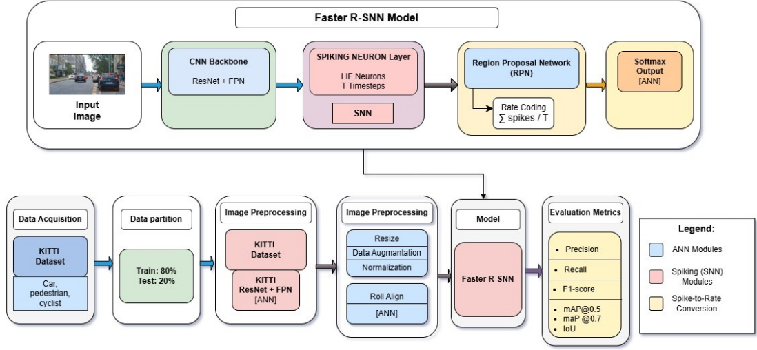
Figure 5.1: R-SNN Architecture Diagram
