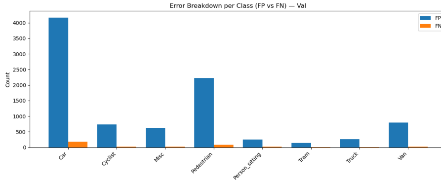
Figure 6.16: False Positive vs False Negative Bar Chart (Faster R-CNN)
