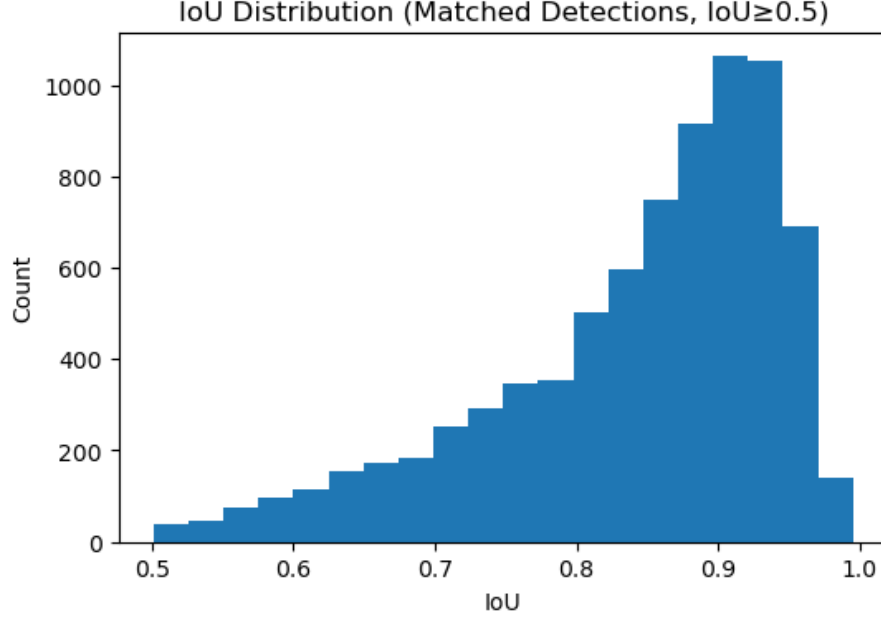
Figure 6.10: Histogram of IoU distribution (Hybrid Model)
