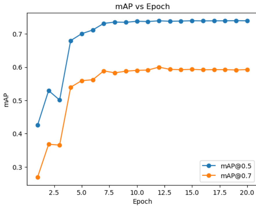
Figure 6.2: mAP vs Epoch (Hybrid Model)
