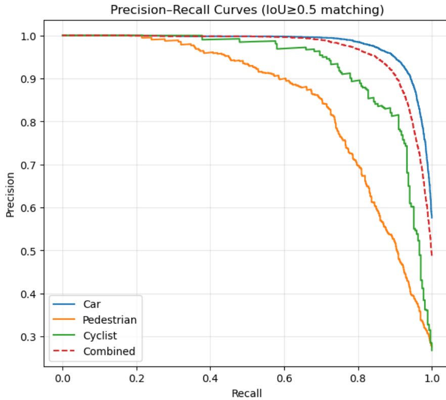
Figure 6.14: Precision-Recall Curves (Faster R-CNN)
