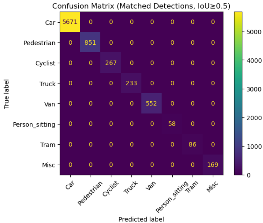
Figure 6.15: Confusion Matrix (Faster R-CNN)
