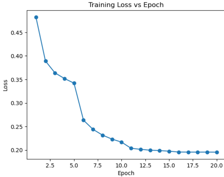
Figure 6.12: Training Loss Vs Epoch (Faster R-CNN)
