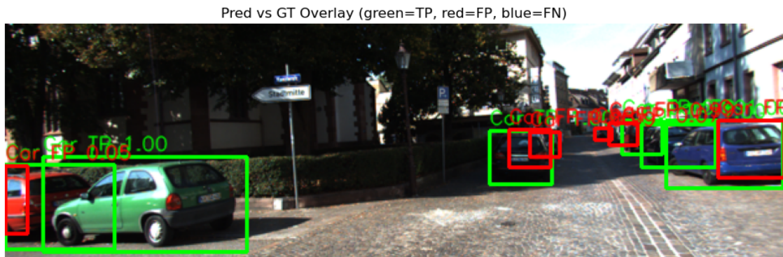
Figure 6.19: Visualization of true positives (TP), false positives (FP) and false negatives (FN) in Faster R-CNN results of detection
