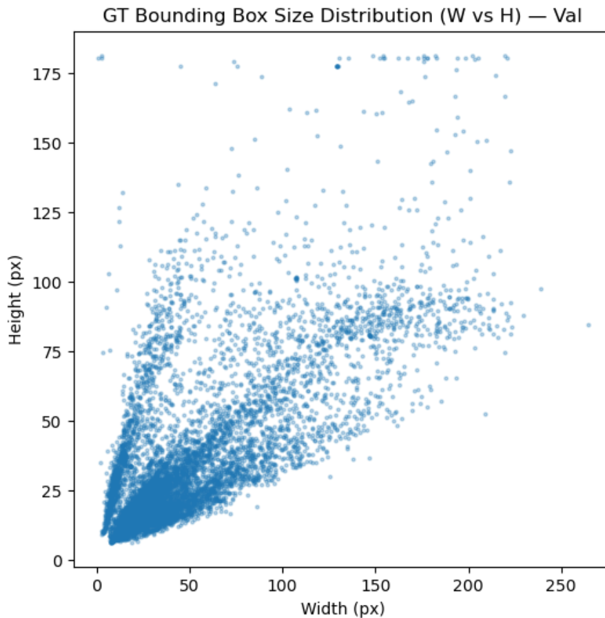
Figure 6.7: Ground truth bounding box size distribution for the KITTI validation set (Hybrid Model)
