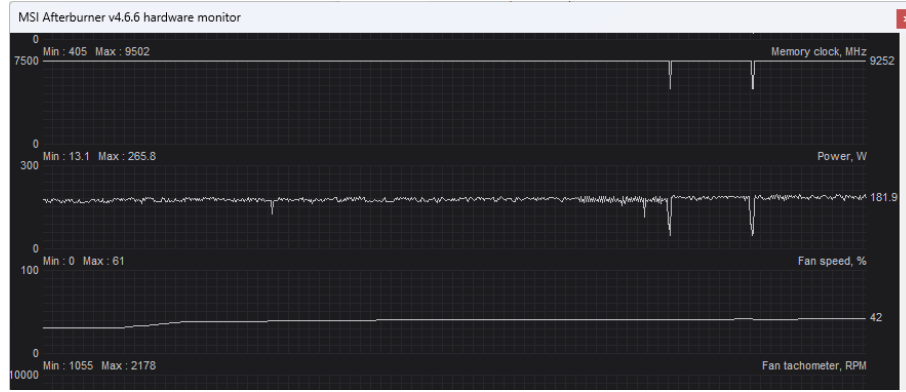
Figure 6.11: Power Consumption (Hybrid Model)
