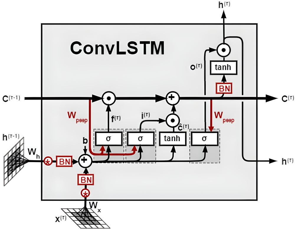
Figure 3.15: Convolutional-LSTM architecture [35]
