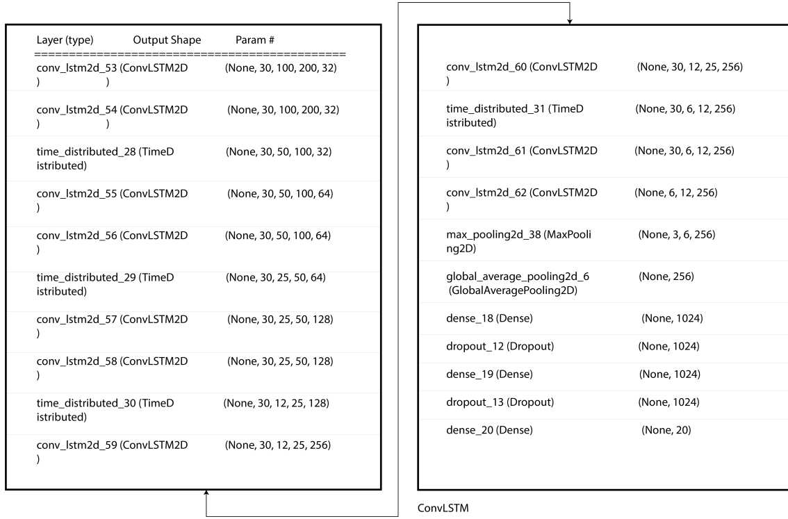
Figure 4.7: Custom ConvLSTM
