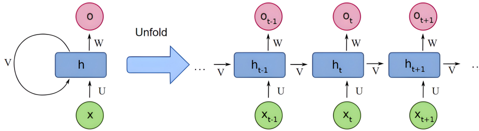
Figure 3.11: RNN Architecture [11]
