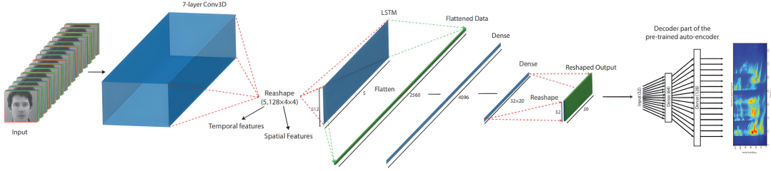
Figure 3.14: Autoencoder-Decoder [17]
