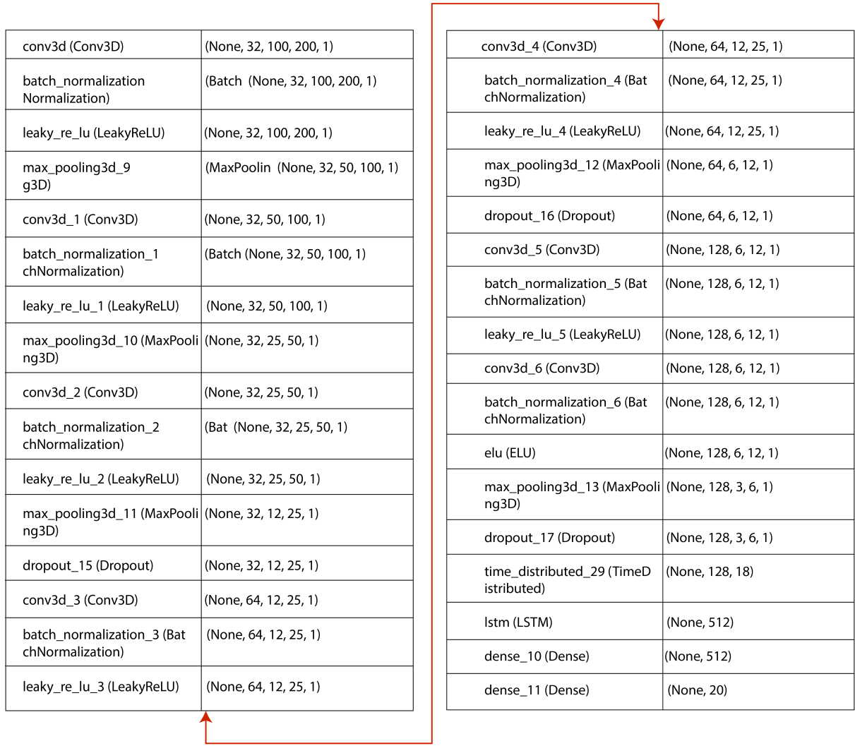
Figure 4.3: Implementation of Autoencoder Decoder model
