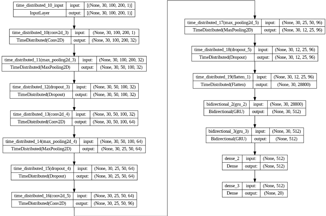
Figure 4.1: Implemented LipNet model details
