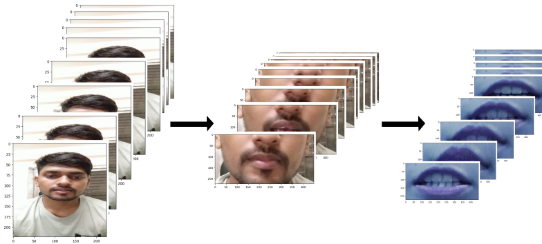
Figure 3.8: Lip segmentation
