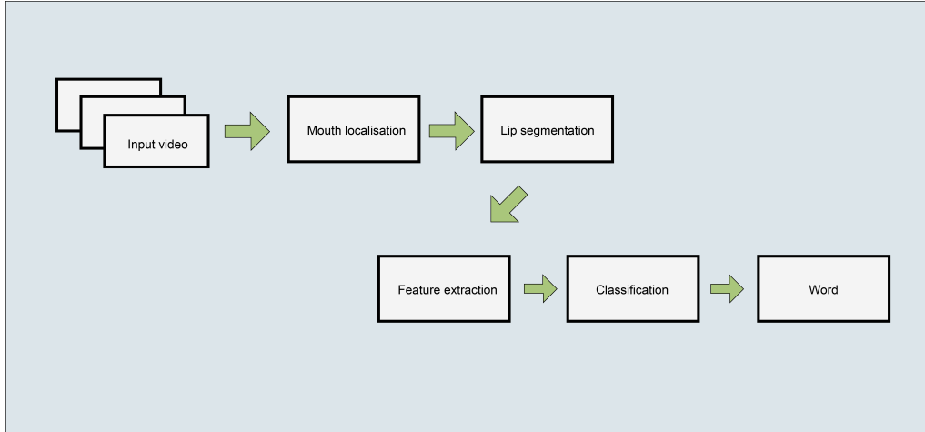
Figure 3.7: Lip-reading processs
