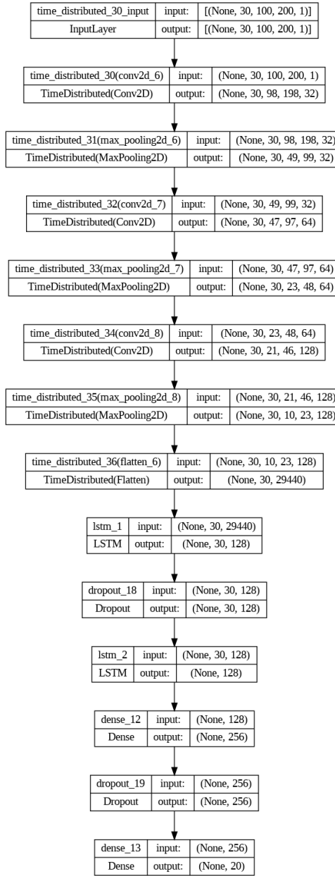
Figure 4.5: Custom CNN-LSTM
