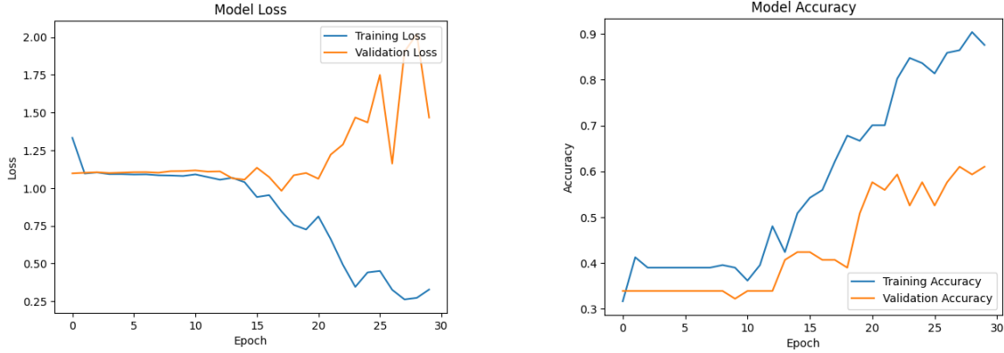
Figure 4.2: Evaluation graph for Lip-Net
