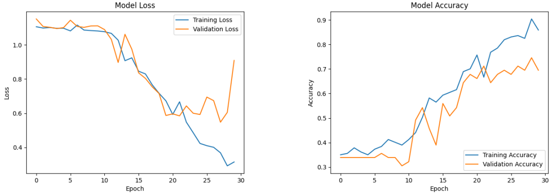
Figure 4.6: Evaluation graph for Custom CNN-LSTM
