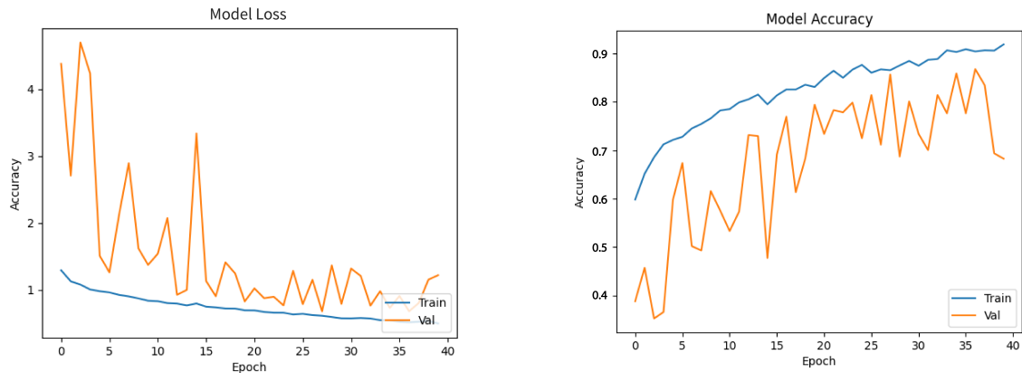
Figure 4.8: Evaluation graph for Custom ConvLSTM
