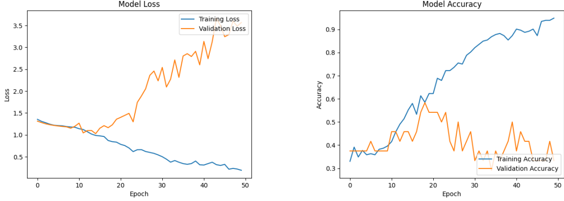
Figure 4.4: Evaluation graph for Auto Encoder-Decoder
