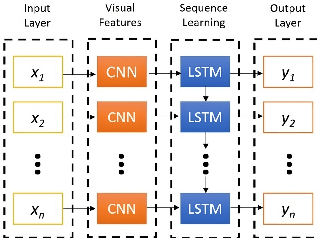
Figure 3.12: CNN-RNN architecture [26]
