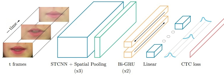
Figure 3.13: LipNet Architecture [12]
