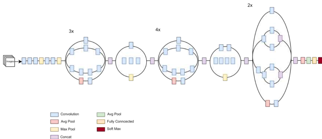
Figure 5.11: Inception-v3 Architecture
