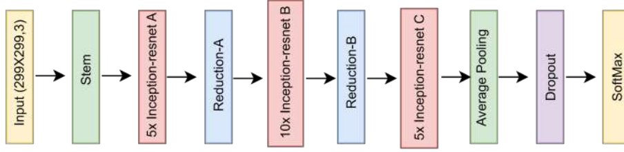
Figure 5.8: Inception-ResNet-v2 Architecture
