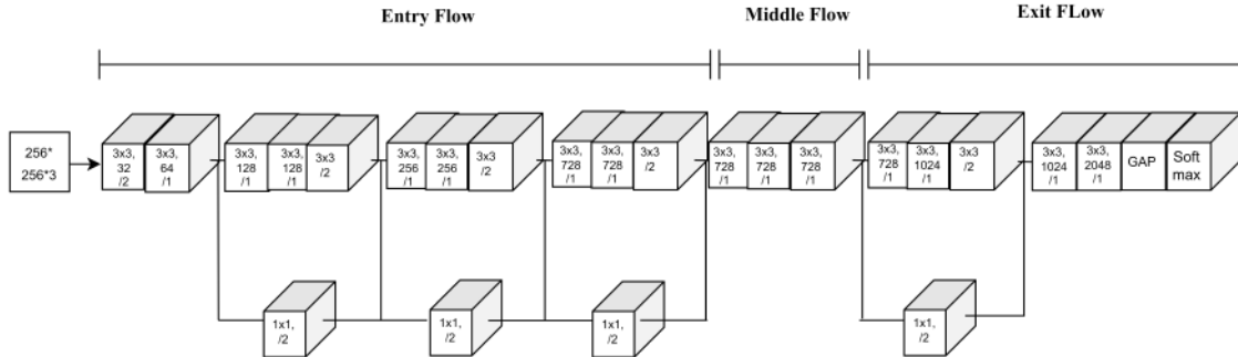
Figure 5.9: Xception Architecture
