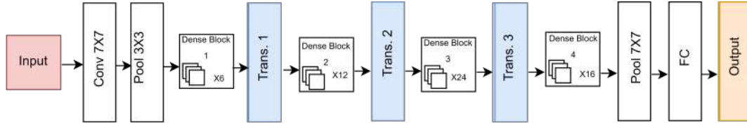
Figure 5.10: DenseNet-121 Architecture
