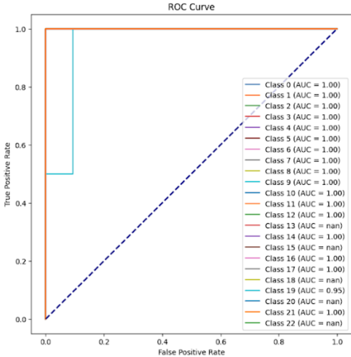
Figure 4.2: ROC Curve
