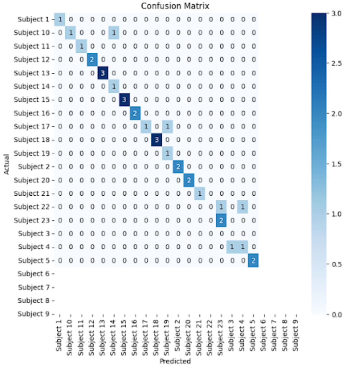
Figure 4.3: Confusion Matrix
