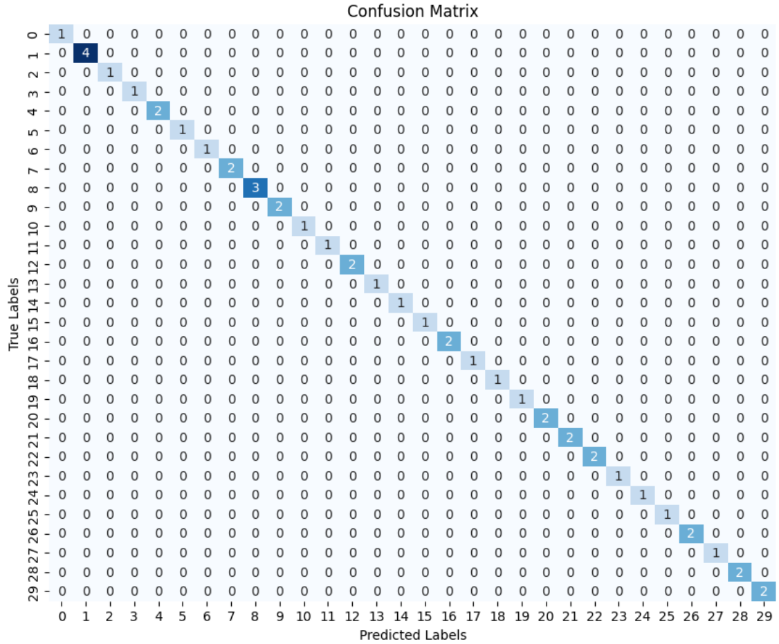
Figure 4.11: Confusion Matrix
