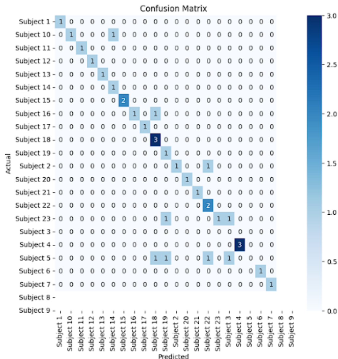
Figure 4.5: Confusion Matrix
