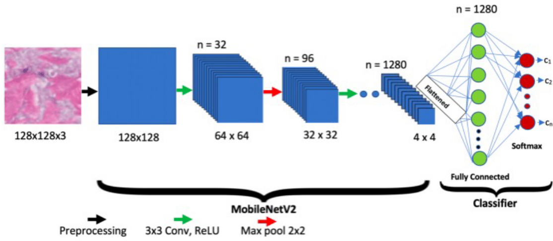
Figure 3.11: MobileNet-V2 Architecture
