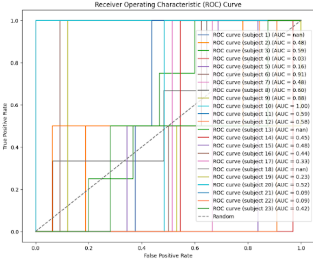
Figure 4.4: ROC Curve
