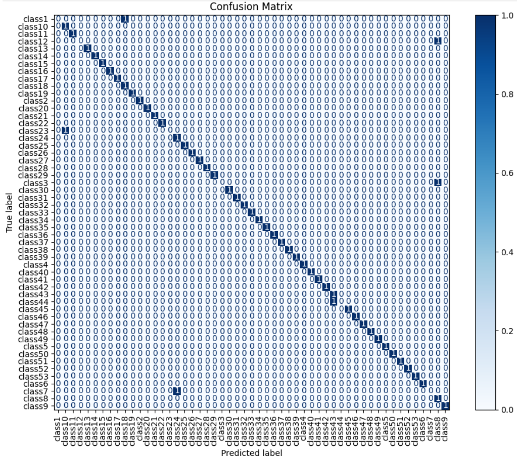
Figure 4.9: Confusion Matrix
