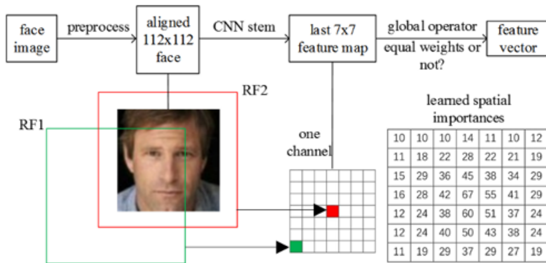
Figure 3.10: MobileFacenet Architecture
