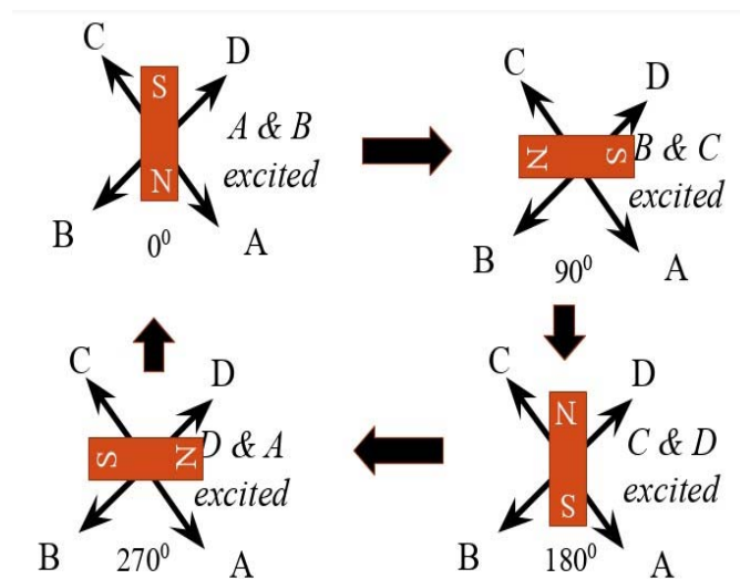
Figure 2.9: Full Step Drive
