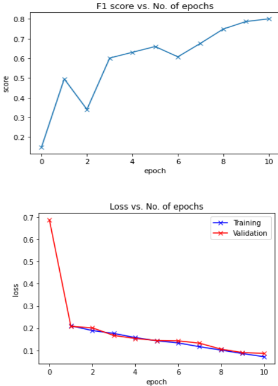
Figure 6.13: Multiple Features Classification Model Accuracy and Loss Graph
