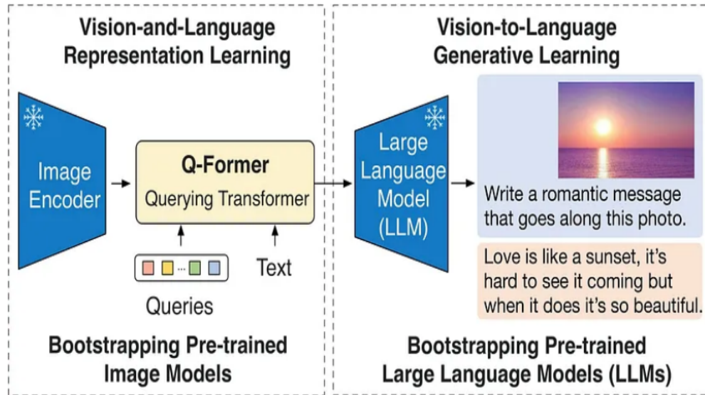
Figure 4.14: Q-Former in BLIP-2 Architecture [32]
