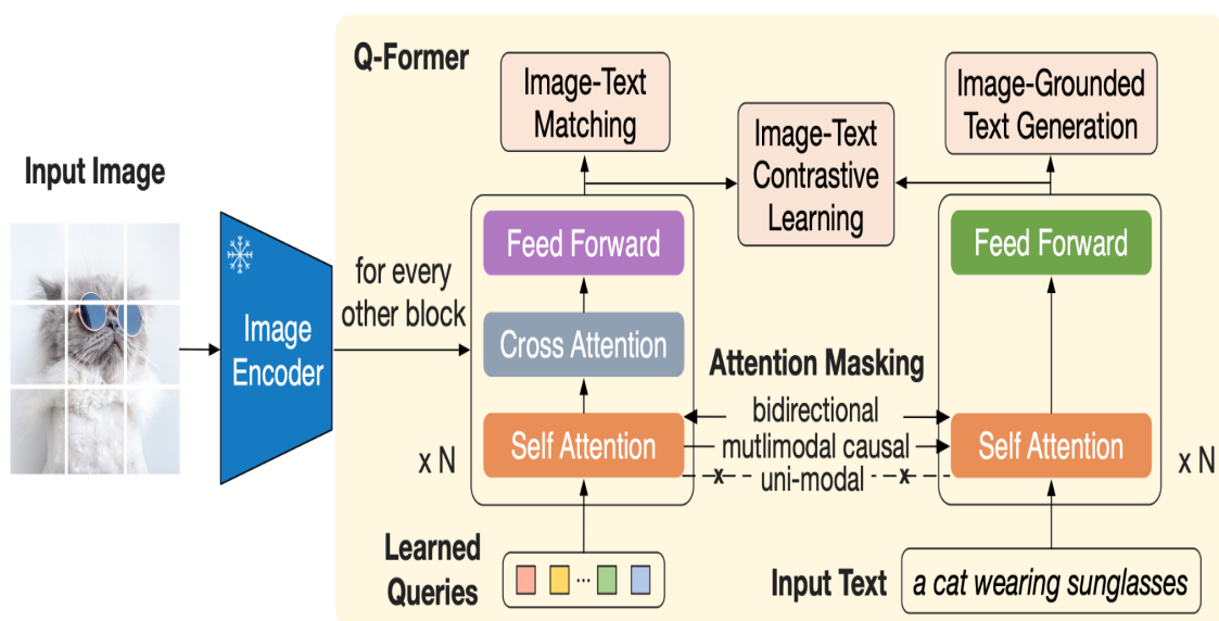
Figure 4.13: BLIP-2 Architecture [32]
