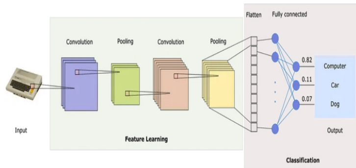
Figure 4.1: CNN Architecture [34]
