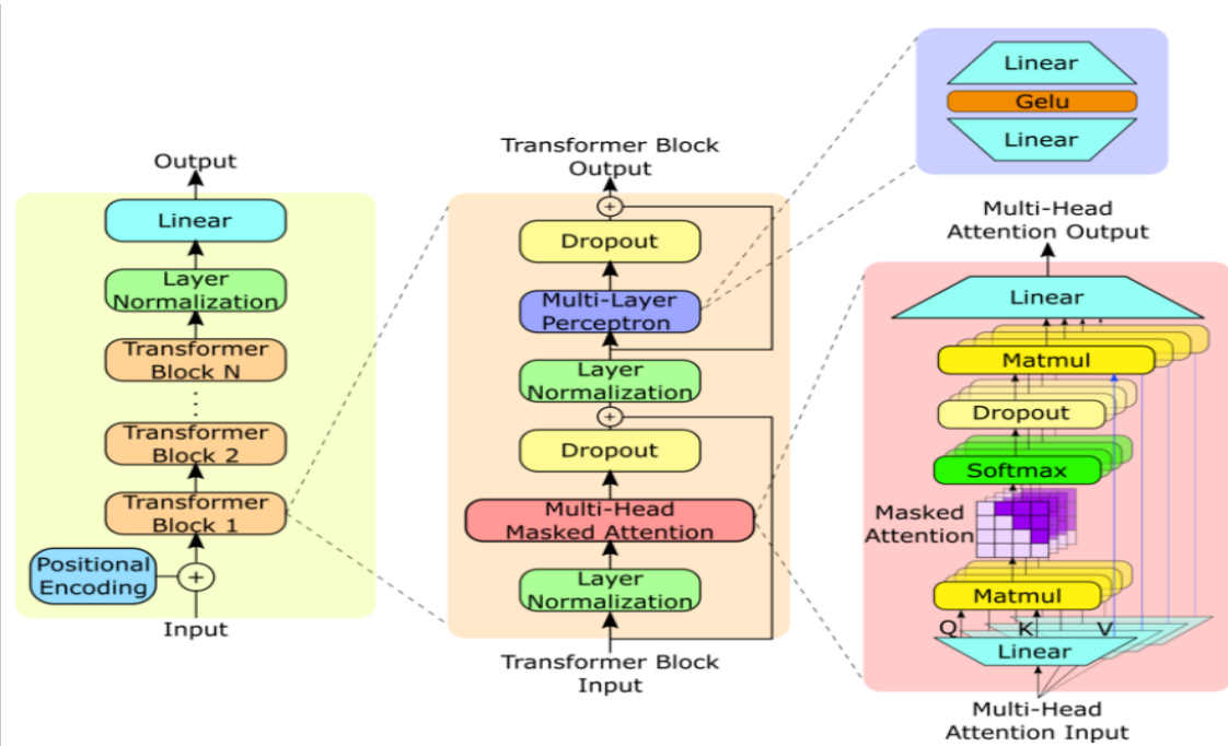
Figure 4.15: GPT-2 Model Architecture [38]
