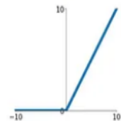
Figure 4.5: Activation Functions [15]
