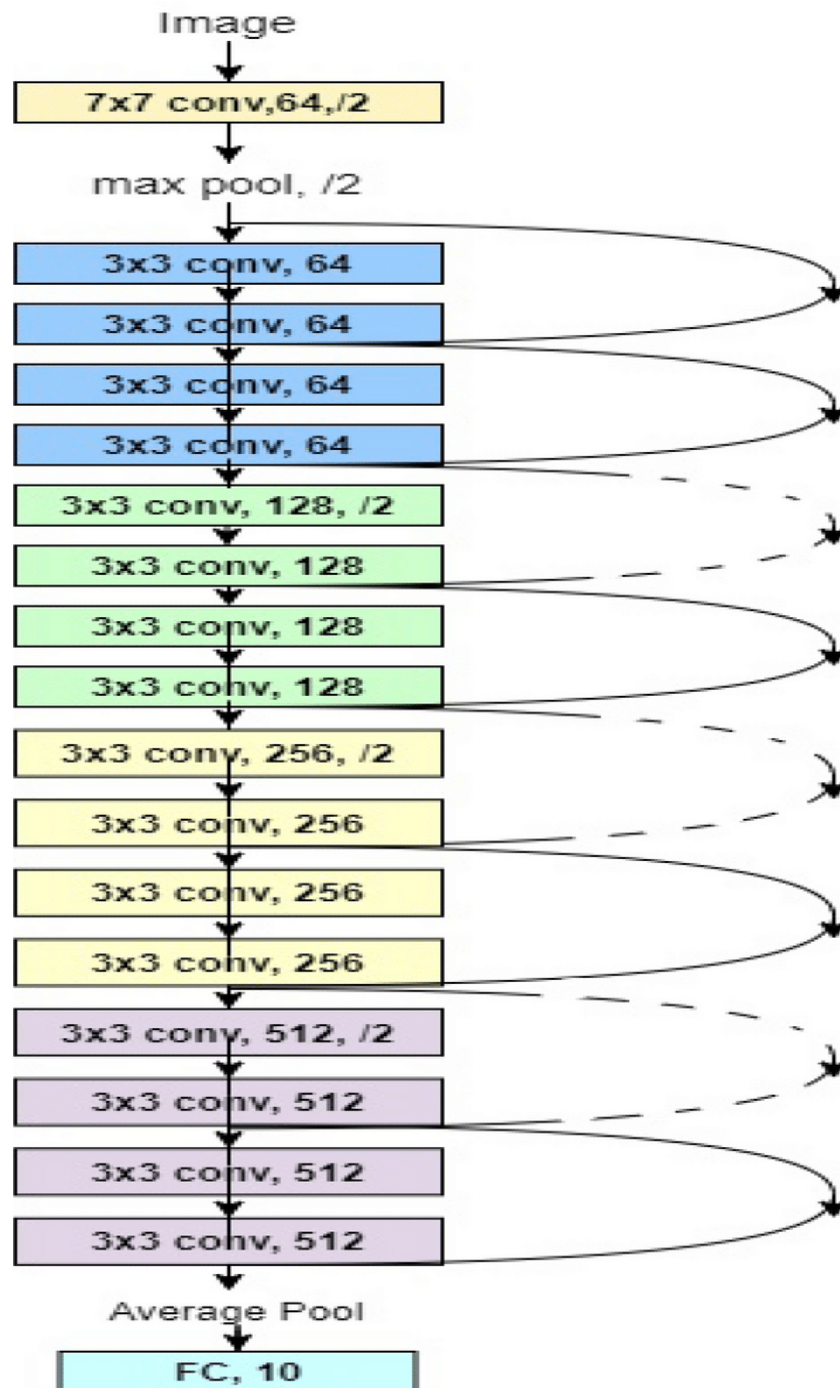
Figure 4.10: ResNet18 architecture [37]
