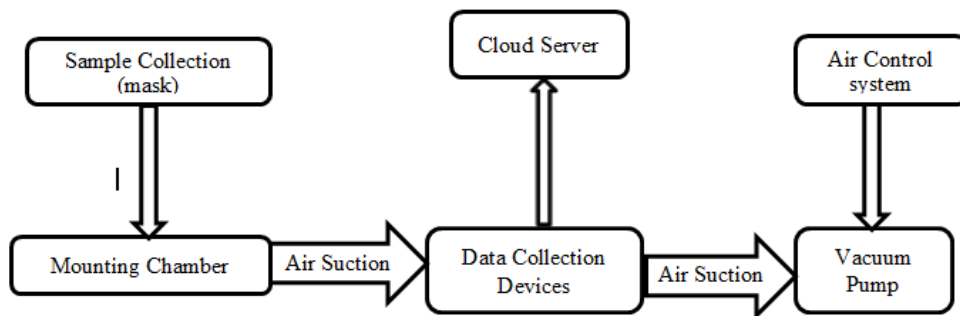
Figure17:Workflow diagram
