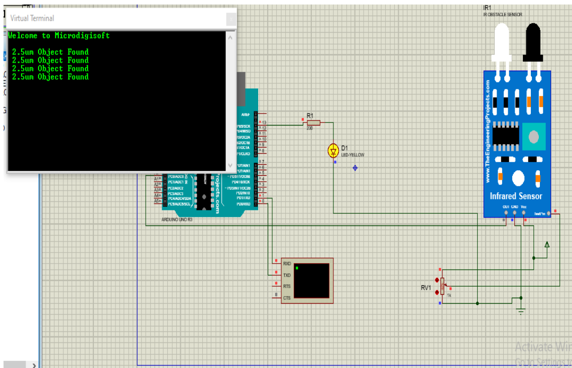
Figure7:Simulation result of Particle Filtration Using IR
