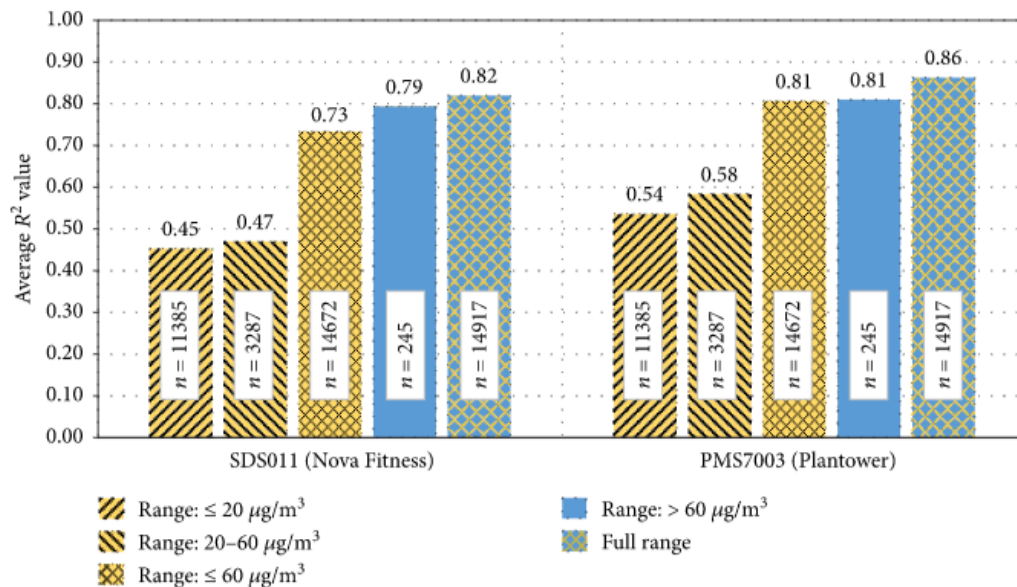
Figure16: Averaged coefficients of determination (R 2 ) for SDS011 and PMS7003 sensors in different concentration ranges for 15 min. n in the text box inside the bar indicates the number of samples used for fitting. Source: Adapted from [21]
