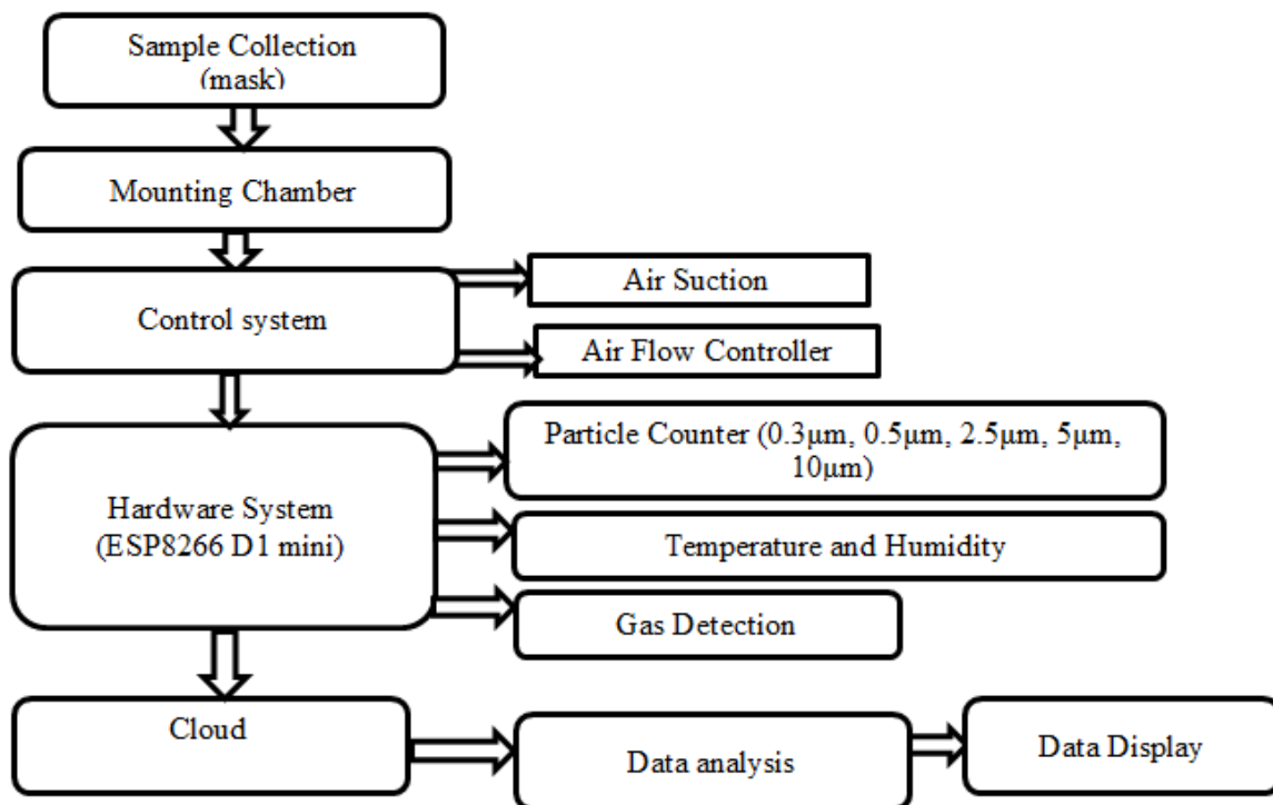
Fig3: IOT Based Particle Filtration
