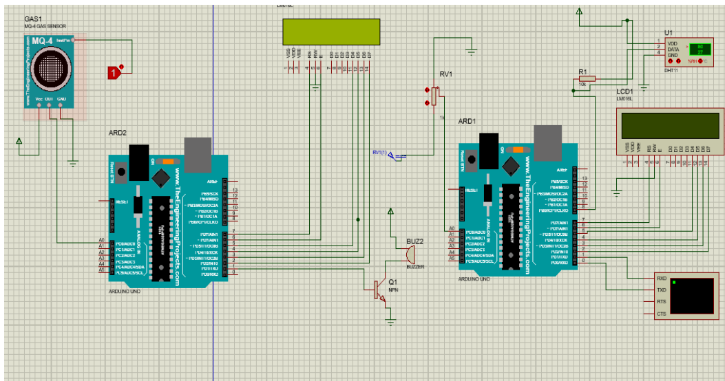
Figure8: Simulation model of Particle filtration with Air Quality Indicator sensor
