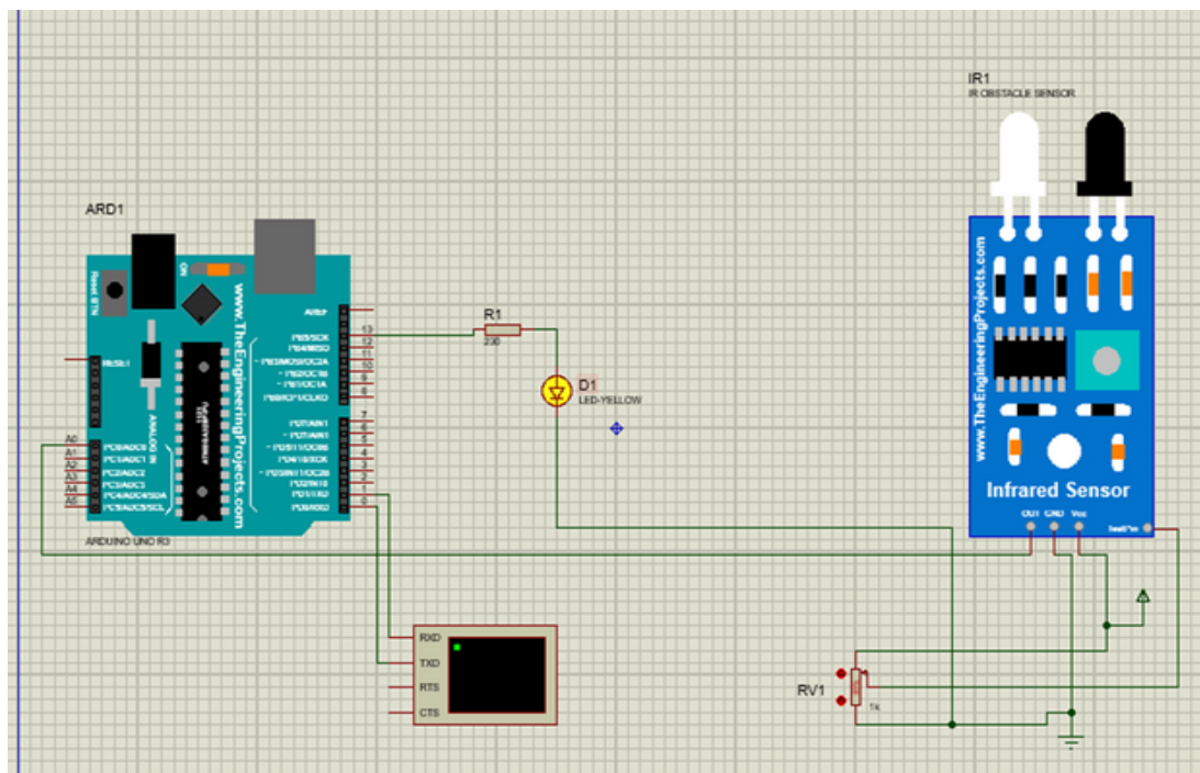
Figure6:Simulation model of Particle Filtration Using IR
