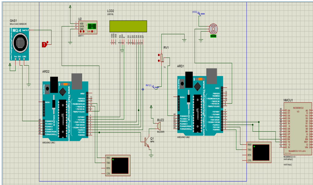
Figure11:Simulation model of IOT Based Particle Filtration
