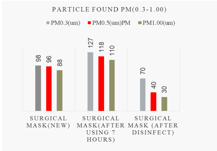
Figure29:Graphical representation of particles for surgical mask(particle size 0.3um-1.00um)
