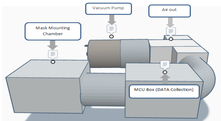
Figure10:3D model of IOT Based Particle Filtration
