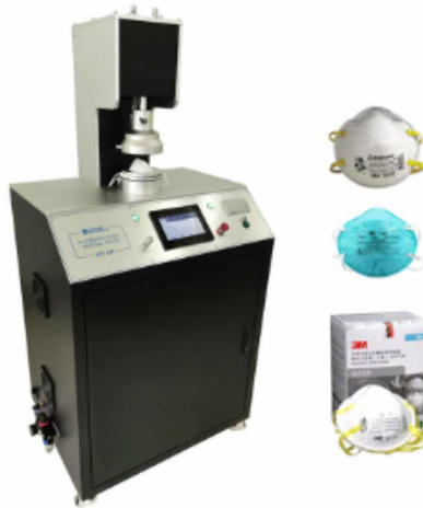
Figure41:Mask Particle Filter Efficiency PFE Tester AFT-100. Source:Adapted from[27]
