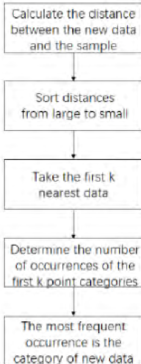
Figure 3.2: KNN[11].
