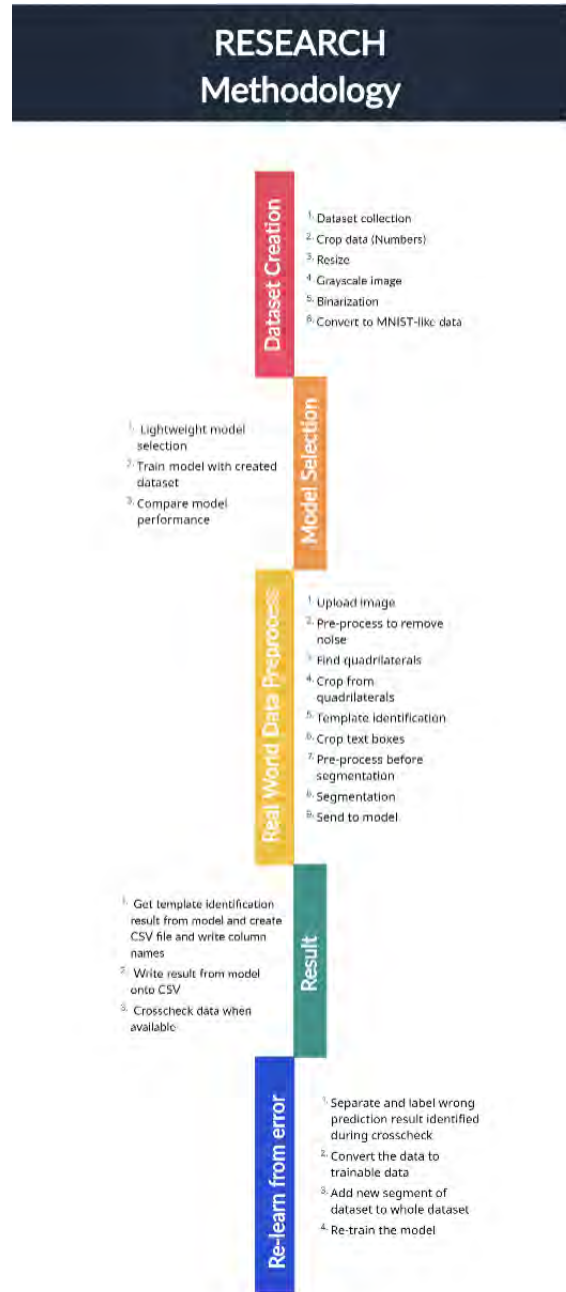
Figure 3.5: Research Methodology.
