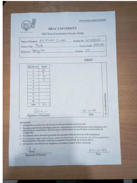
Figure 5.3: Test Script.
