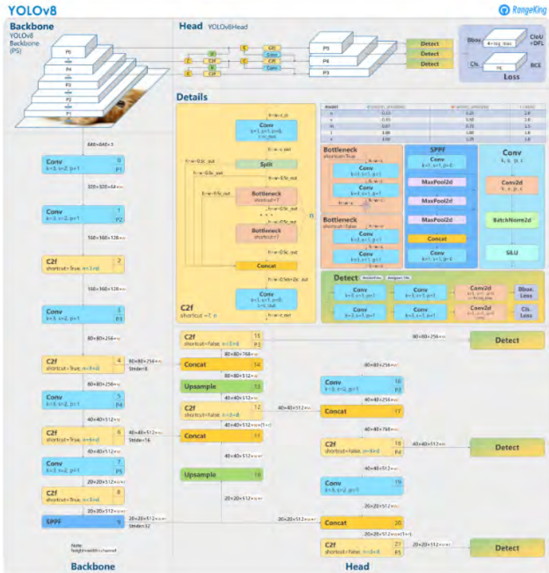
Figure 3.3: YOLO [19].
