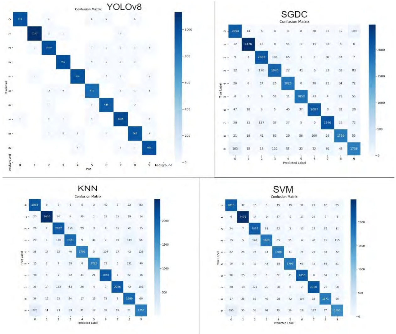
Figure 6.1: Confusion Matrix of Different Models.
