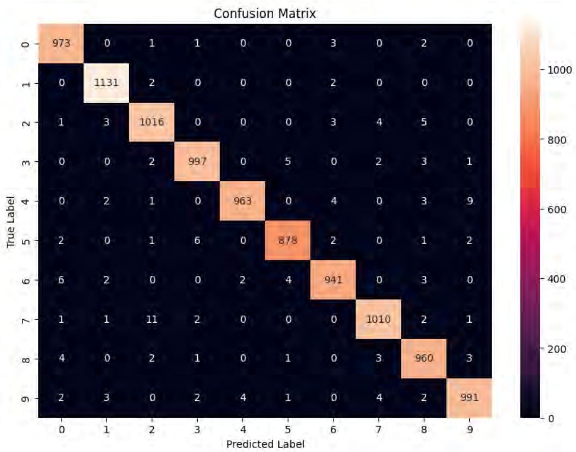
Figure 6.2: Confusion Matrix of CNN.
