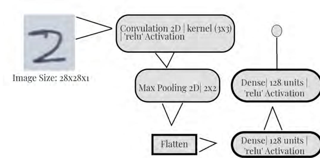
Figure 3.1: CNN.
