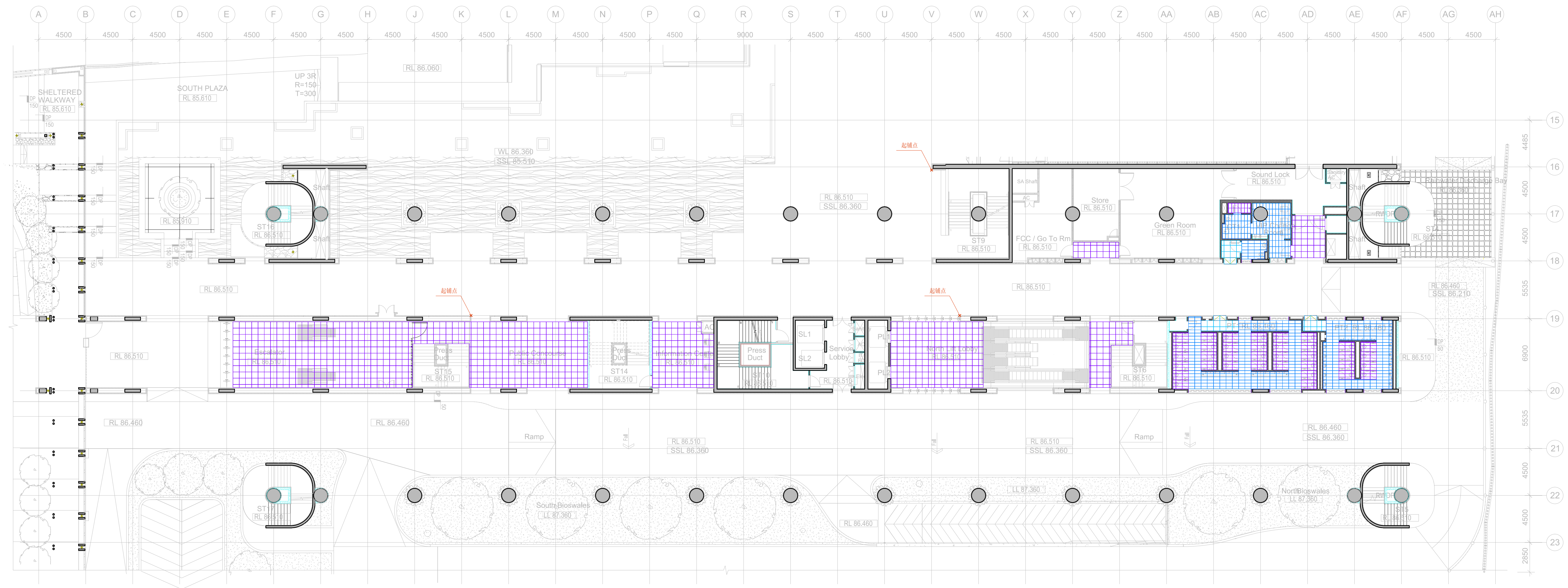
1 GF Layout of Tiles(East Wing) 1:200
