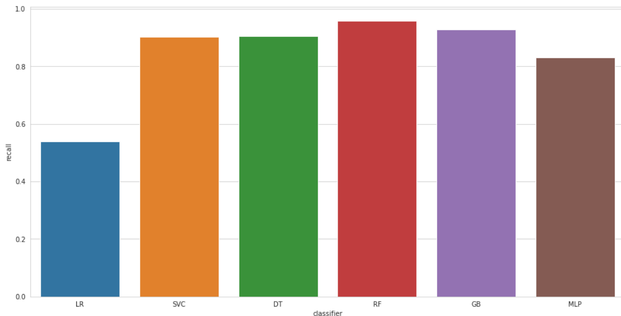
Figure 6.15: Recall Analysis
