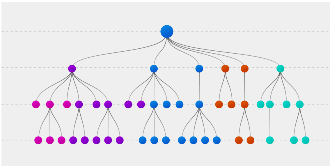
Figure 5.5: Decision tree [63]
