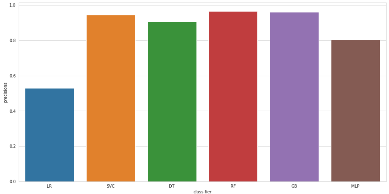
Figure 6.14: Precision Analysis
