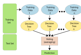
Figure 3.3: Working of RF Algorithm.[23]
