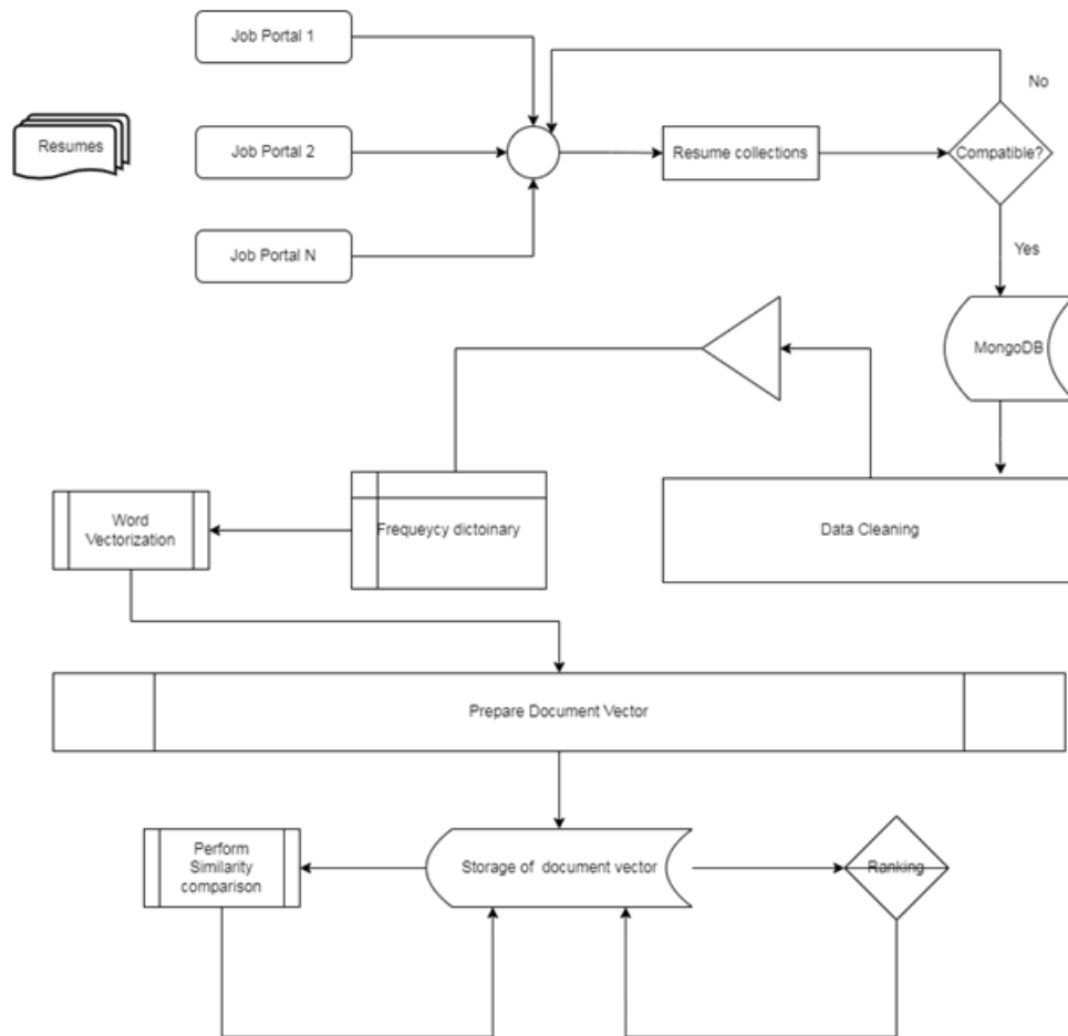
Figure 3.3: Process flow diagram for background process
