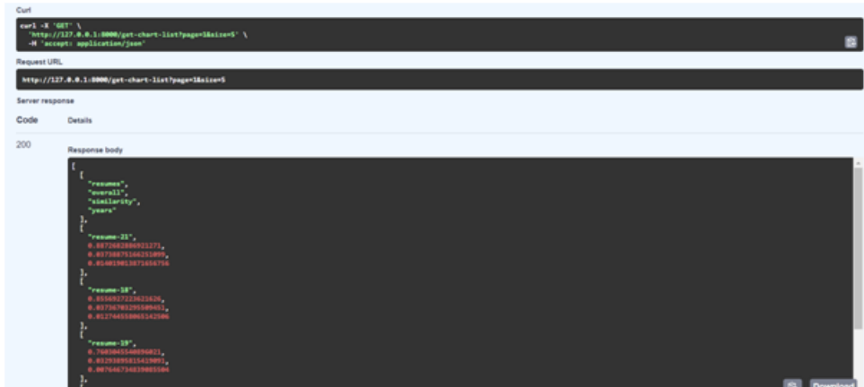
Figure 7.4: API request response sample
