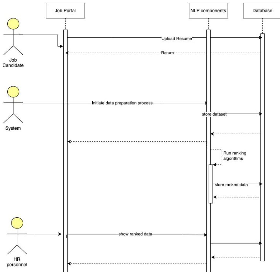
Figure 3.5: Actor-system sequence diagram
