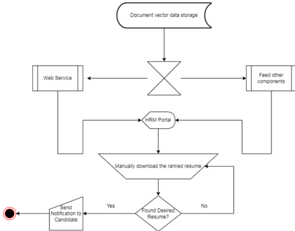
Figure 3.4: Process flow diagram for foreground process
