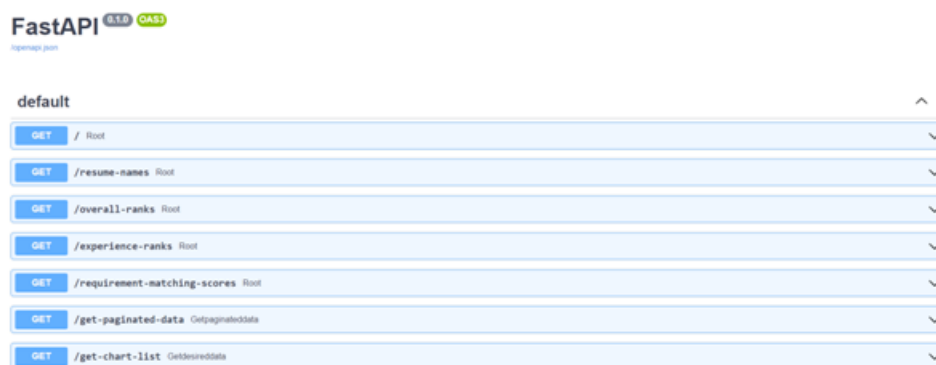
Figure 7.3: API Document
