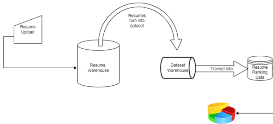
Figure 3.6: Dataflow diagram
