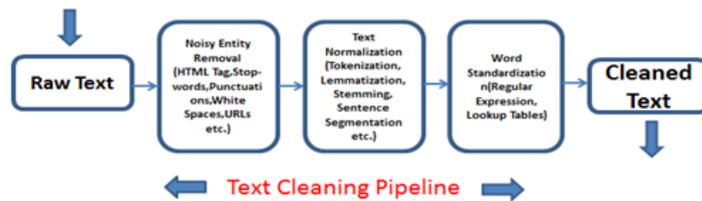
Figure 2.2: Text pre-processing
