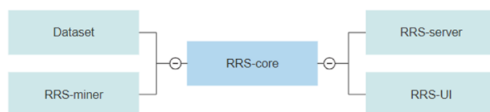
Figure 1.1: System Components
