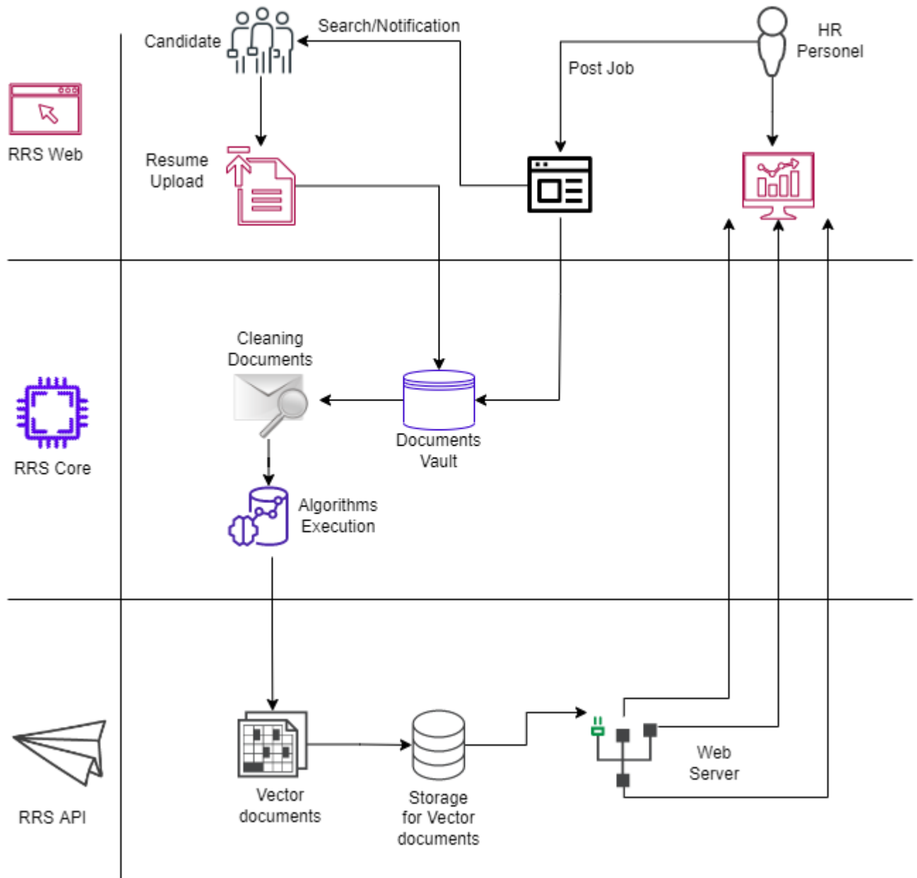
Figure 3.2: RRS architectural diagram
