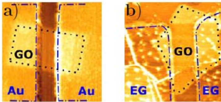
Fig4: a) a bilayer rectangular GO flake (outlined by a black dotted line) over a 400nm Au gap. Blue dash dot lines represent Au pads. b) A pentagonal GO flake bridges 2 EG electrodes 11 .
