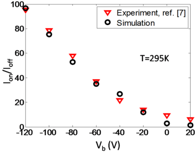
Fig-10: On/off current ratio as a function of the back gate bias voltage ( V_b ). Experimented values almost match the simulation values. There's only a slight mismatch between the experimented and simulated values 15 .
