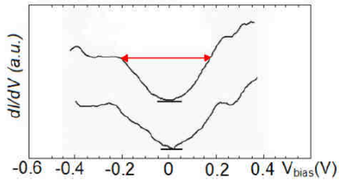
Fig9: STS spectra of a narrow ribbon revealing an energy gap of about 0.5 eV. (fig is taken from ref.10.)
