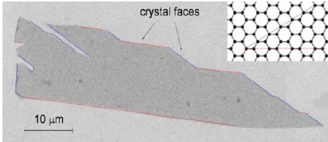
Fig8. Scanning-electron micrograph of a relatively large graphene crystal, which shows that most of the crystal's faces are zigzag and armchair edges as indicated by blue and red lines 2
