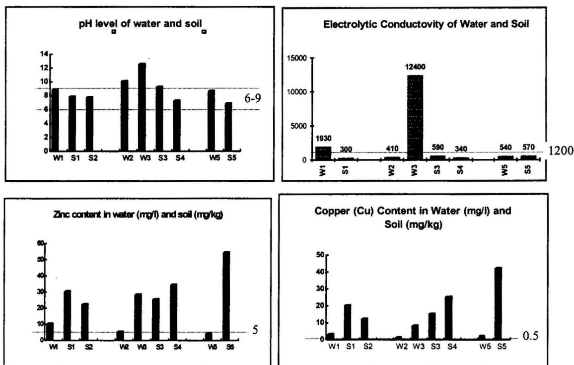
Figure 1: Comparison of Chemical Contents in Water and Soil Sample at Different Sites of Sericulture and AAF (dotted lines parallel to x-axis indicate the DoE standard for inland surface water)
