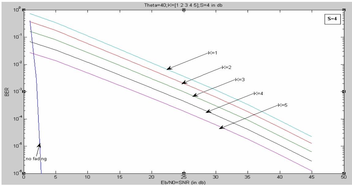
Graph 7: Angle 40^{\circ} ; Shadowing 4db & Rice factor 1, 2,3,4,5
